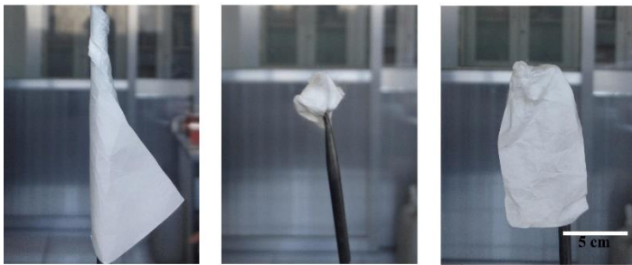
Figure S3. The flexibility test of PAN@PVDF-HFP separator. No cracks or pin-holes can be easily found after being rolled up or scrunched several times.
