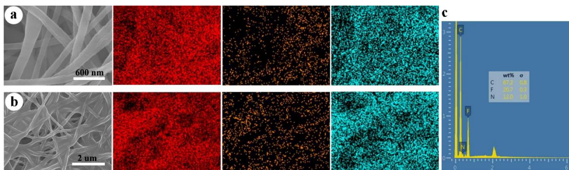
Figure S7. Elemental mapping of selected area of PAN@PVDF-HFP fiber network: (a) Elemental mapping at room temperature and (b) at 180 °C; (c) EDS results.
