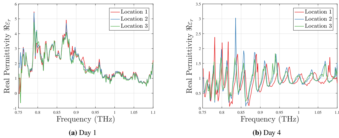
Figure 3. Real part of permittivity of coffee leaves at three different locations taken on days 1 and 4.
