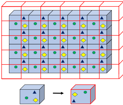
FIG. 1: While the positions of the particles inside a crystal are fixed, all the cells as a whole can be translated anywhere together, then be placed in the new position. The red frame is an example of the new cell placement. In the lower part of this figure, the yellow diamond particle in the right-bottom corner of the old cell on the left, is in the top-left corner of the new red-framed cell on the right now, viewed through the front surfaces.
