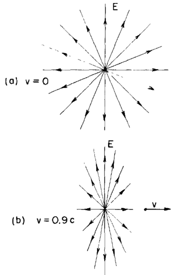
Figure 2 - (from Feynman[5]) The bunching of field lines in the direction of motion of the charge.
