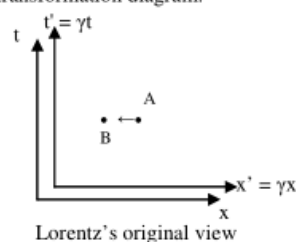
Figure 1 - Removal of the retarded time terms from the Lorentz Transform leads to Absolute Space and Time.
