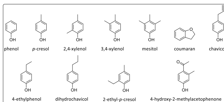
Figure 10. Detected Py-GC/MS fragments attributed to the H-unit.
