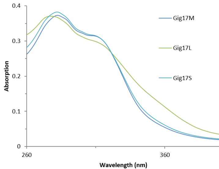
Figure 8. UV/Vis curves for lignins obtained from Miscanthus x giganteus . (mixture: Gig17M; leaf: Gig17L; stem Gig17S).
