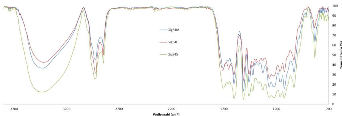
Figure 5. FT-IR spectra of mixture (Gig34M), leaf (Gig34L) and stem-derived (Gig34S) lignins obtained from M. x giganteus (Gig34).
