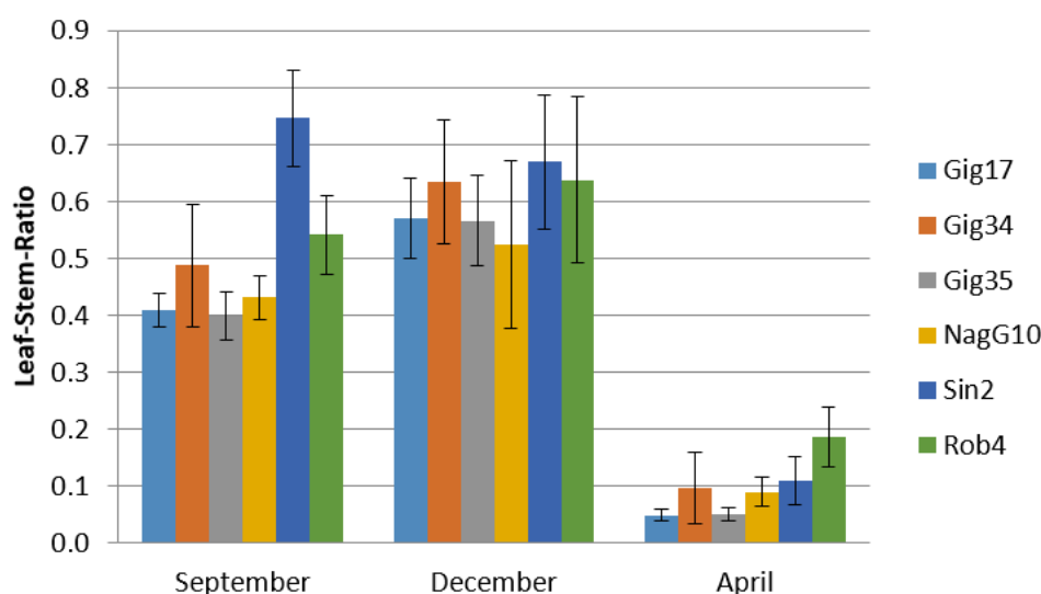
Figure 2. Miscanthus crop analysis via NREL measurements. Leaf versus stem content of Miscanthus genotypes: M. x giganteus (Gig17, Gig34, Gig35), M. nagara (NagG10), M. sinensis (Sin2) and M. robustus (Rob4) harvested in September (09/15), December (12/14) and April (04/15), respectively (arranged to follow the seasonal order from autumn to spring).
