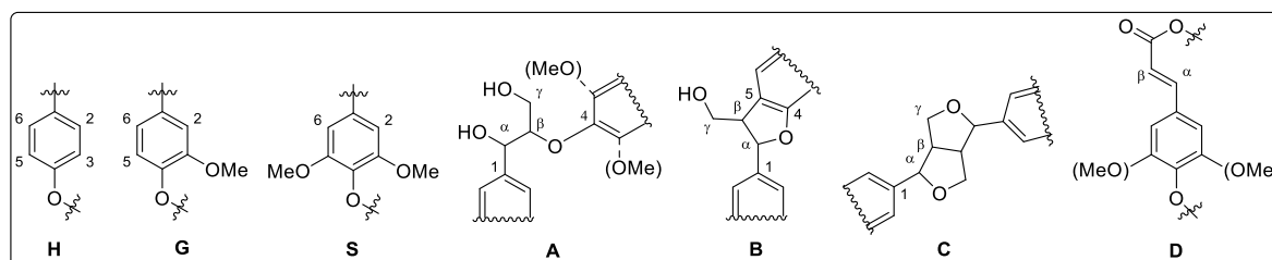
Figure 15. Lignin structure elements for HSQC NMR signal assignment (A: \beta -O-4 linkage, B: phenylcoumaran, C: resinol, D: \beta -unsaturated ester).
