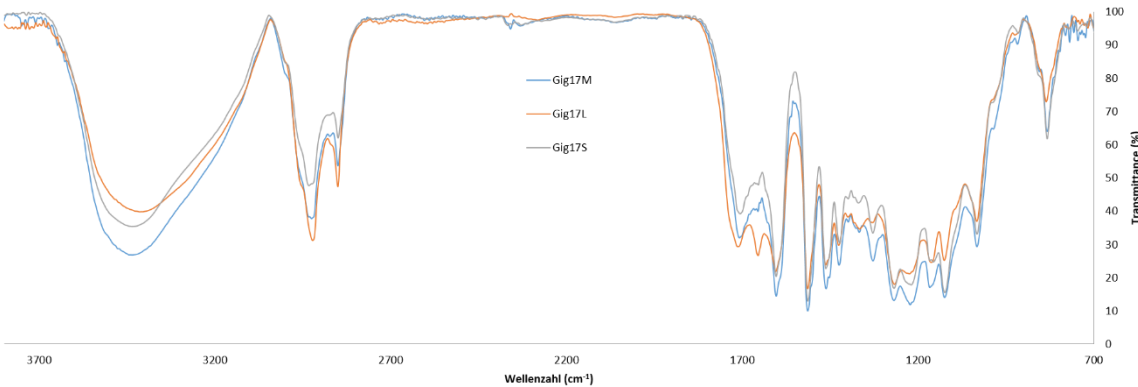
Figure 4. FT-IR spectra of mixture (Gig17M), leaf (Gig17L) and stem-derived (Gig17S) lignins obtained from M. x giganteus (Gig17).
