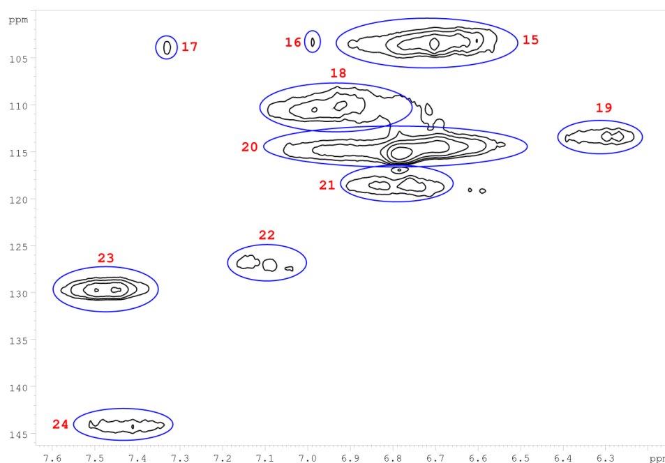
Figure 14. Aromatic HSQC region of a lignin obtained from M. X giganteus stem/leaf mixture (Gig17M). Numbers are listed and assigned in Table 9.
