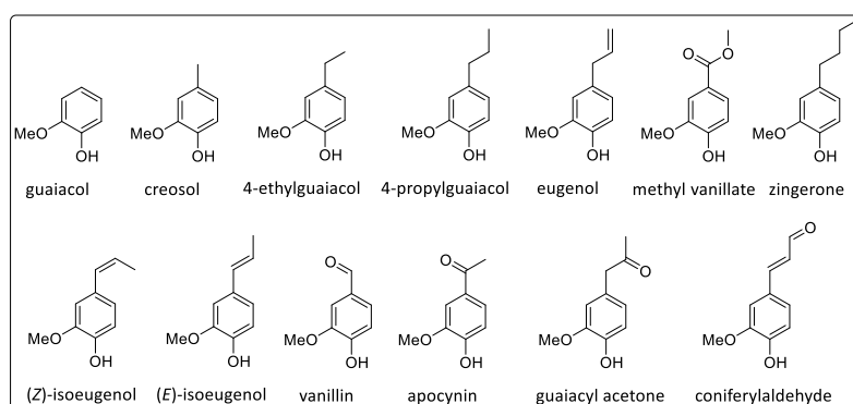
Figure 11. Detected Py-GC/MS fragments attributed to the G-unit.
