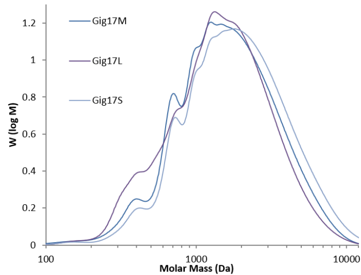
Figure 7. SEC curves of lignins obtained from Miscanthus x giganteus (mixture: Gig17M; leaf: Gig17L; stem Gig17S).
