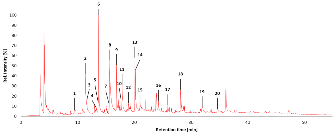
Figure 9. Pyrolysis-GC/MS pyrogram of a lignin obtained from Miscanthus x giganteus Gig17M. (stem/leaf mixture) with numbers for all aromatic fragments listed and assigned in Table 6.
