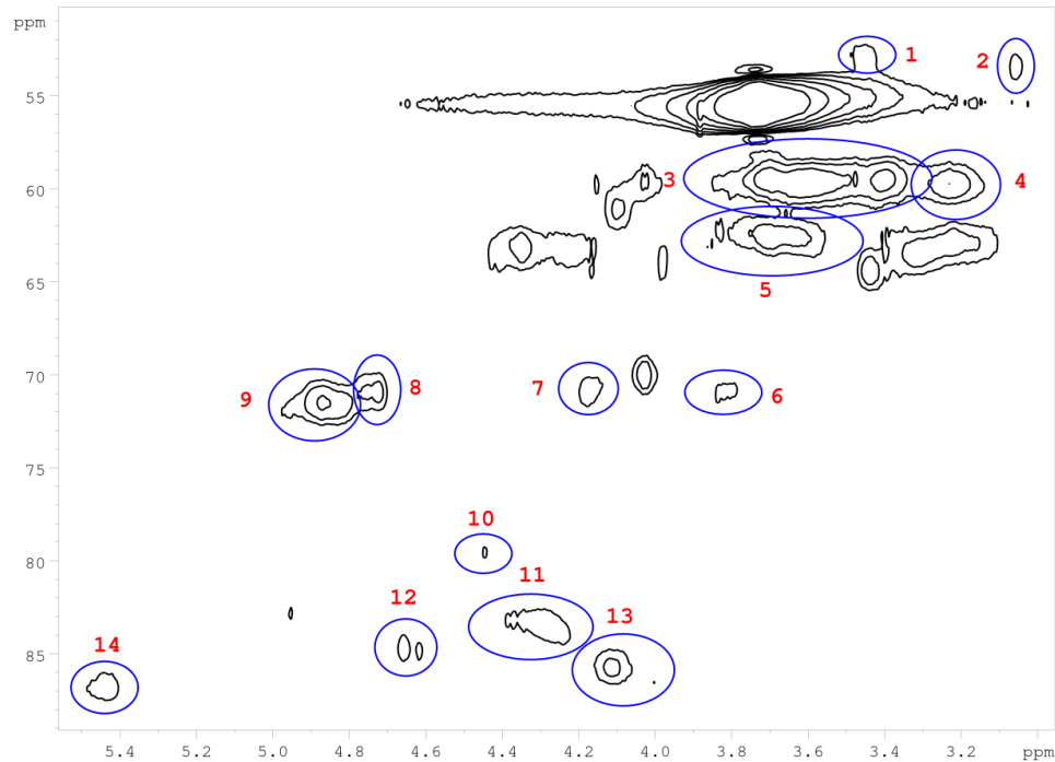
Figure 13. Non-aromatic HSQC region of a lignin obtained from M. X giganteus stem/leaf mixture (Gig17M). Numbers are listed and assigned in Table 9.
