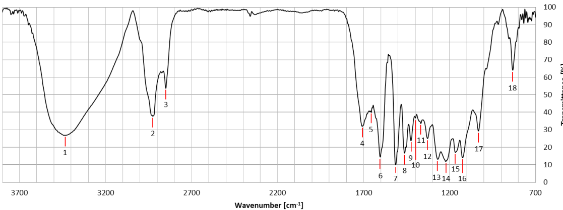
Figure 3. FT-IR spectra of Gig17 (stem, leaf and mixture) with numbered signals listed in Table 4.
