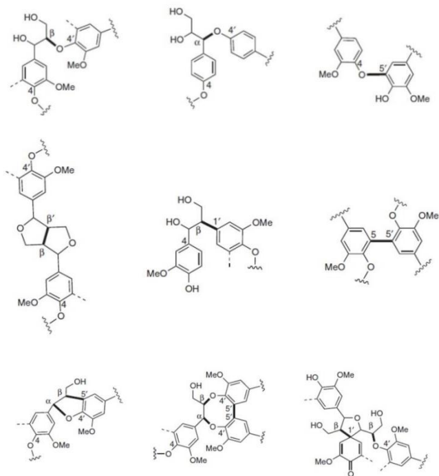
Figure 1. Monolignol linkages. First line: Ether bonds ( \beta -O-4', \alpha -O-4', 4-O-5'); second line: C-C-bonds. ( \beta - \beta' , \beta -1', 5-5'), and third line: more complex linkages ( \beta -5'/ \alpha -O-4', 5-5'/ \beta -O-4'/ \alpha -O-4', \beta -1'/ \beta -O-4').
