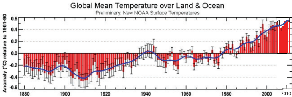
FIG. S1: Changes in global mean surface temperature relative to 1961–2013 (source: NOAA).
