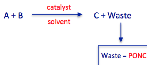
Figure 1. Any waste in a chemical reaction used by industry to afford the desired product (C) adds to the overall price of nonconformity (PONC) paid by the company.
