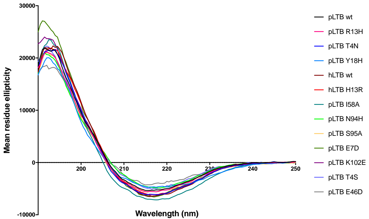
Figure S1. Circular dichroism of pLTB and hLTB variants discussed in the paper, showing that they are folded.
