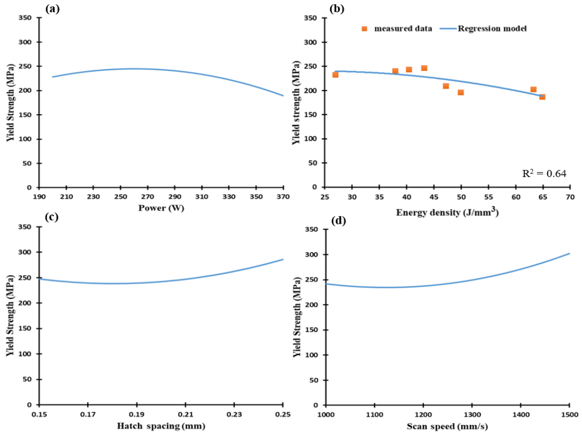
Figure 15. Yield strength of the as-built AlSi10Mg samples vs. a) Laser power (W), b) Energy density (J/mm³), c) Hatch Spacing (mm), and d) Scan speed (mm/s).
