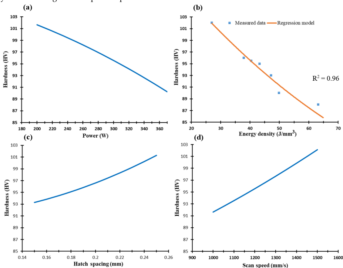
Figure 10. Microhardness of the as-built AlSi10Mg samples along the Z-direction vs. a) Laser power (W), b) Energy density (J/mm 3 ), c) Hatch spacing (mm), and d) Scan speed (mm/s).
