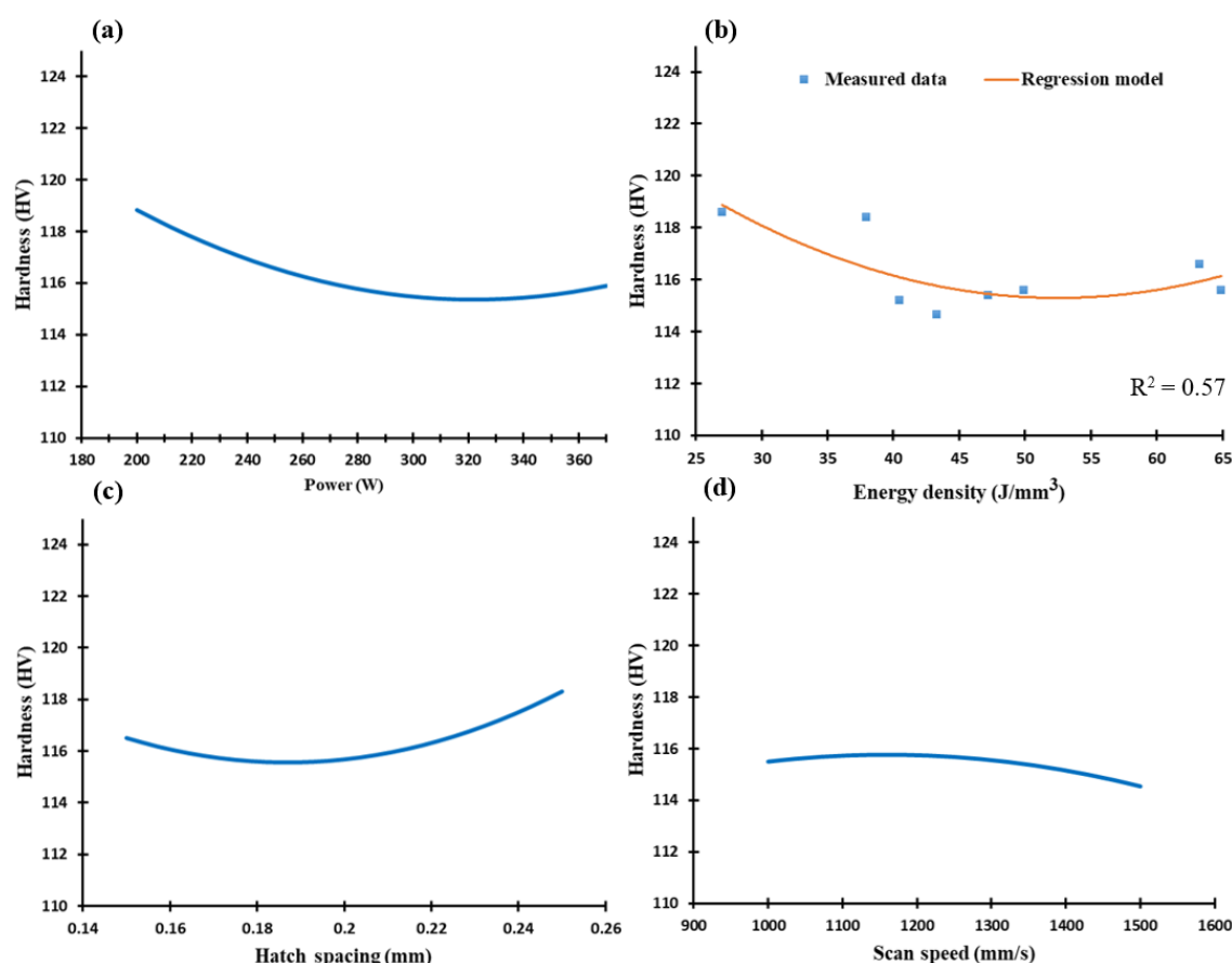
Figure 11. Microhardness of the as-built AlSi10Mg samples along the XY plane vs. a) Laser power (W), b) Energy density (J/mm 3 ), c) Hatch spacing (mm), and d) Scan speed (mm/s).
