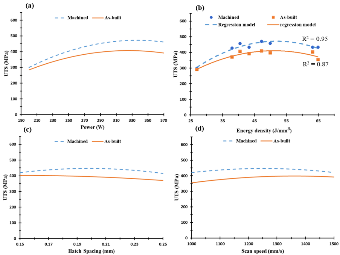
Figure 14. Ultimate tensile strength of the as-built AlSi10Mg samples along the building direction vs. a) Laser power (W), b) Energy density (J/mm³), c) Hatch Spacing (mm), and d) Scan speed (mm/s).
