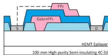
Fig. 1 Schematic cross section of the AlGaIn/AlN/GaN structure
