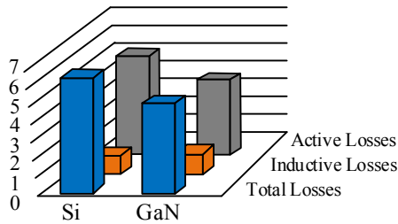
Fig. 8 Converter Losses
