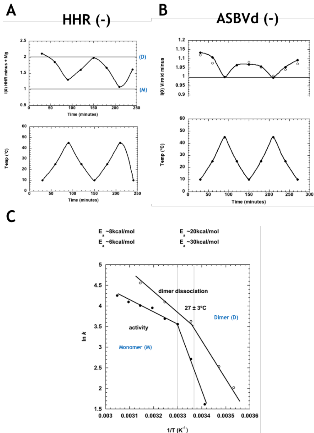
Figure 3. (A) Normalized forward scattered SANS intensity for HHR (-) in presence of Mg ++ at the corresponding temperature on the plot below. The values at 1.00 and 2.00 correspond to the intensity expected for the monomer (M) and dimer (D), respectively. (B) Normalized forward scattered SANS intensity for ASBVd (-) in presence (filled circles) and absence (open circles) of Mg ++ , at the corresponding temperature on the plot below. The data indicate a small amount of dimer formation at the lower temperature. (C) Arrhenius plots of HHR (-)/Mg rate of dimer dissociation (open circles, calculated from (A)), and the ribozyme's catalytic activity (filled circles), revealing parallel behaviour. Modified from Leclerc et al. [33].
