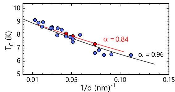
Figure 4. Top) Superconducting transition temperature as a function of the reciprocal film thickness. Blue circles are Nb films on \text{SiO}_2 substrate and red circles on sapphire substrate. Continuous line is least-squares fit, using Eq. (1). The effective thickness of the normal layer (in nm) is represented by the corresponding \alpha value. Bottom) Plot of the ratio T_c/F(d) as a function of the film thickness. The fitting function, F(d) , has been calculated using the theoretically expected value of the Nb bulk transition temperature (i.e. T_{C0} = 9.22 K).
