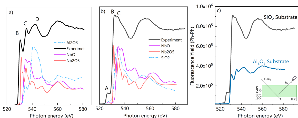
Figure 3. X-ray absorption near edge (XANES) spectra of the O K-edge of the films deposited on the a) sapphire and b) silicon oxide in total fluorescence yield mode along with the reference spectra of \text{SiO}_2 , \text{Al}_2\text{O}_3 , \text{Nb}_2\text{O}_5 and \text{NbO} . c) normalized fluorescence yield, measured on samples on \text{SiO}_2 and sapphire along with the MPD of the TFY schematic. The overall yield error was estimated of the order of 1%.
