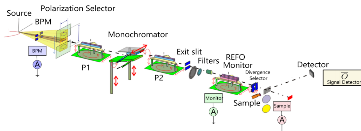
Figure 1. BEAR beamline set up [17].
