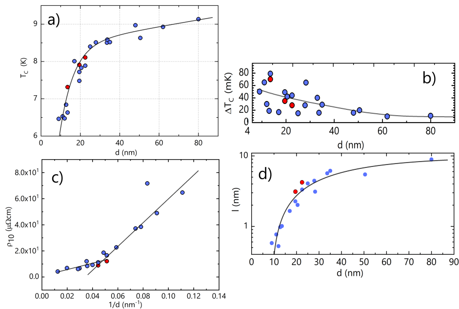
Figure 2. Thickness dependence of a) T_C on the thickness of Nb films deposited on \text{SiO}_2 (blue) and sapphire (red); b) The superconducting transition width. Red circles are Nb Films on sapphire. Continuous line is a guide for eyes; c) The residual resistivity for films on \text{SiO}_2 and sapphire; and d) The mean free path at 10 K. Data have been derived from the resistivity values measured at the same temperature (i.e. \rho_{10} ).
