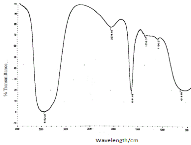
Fig. 3: FTIR spectra of local textile wastewater Treated with Bacillus licheniformis Zul 012
