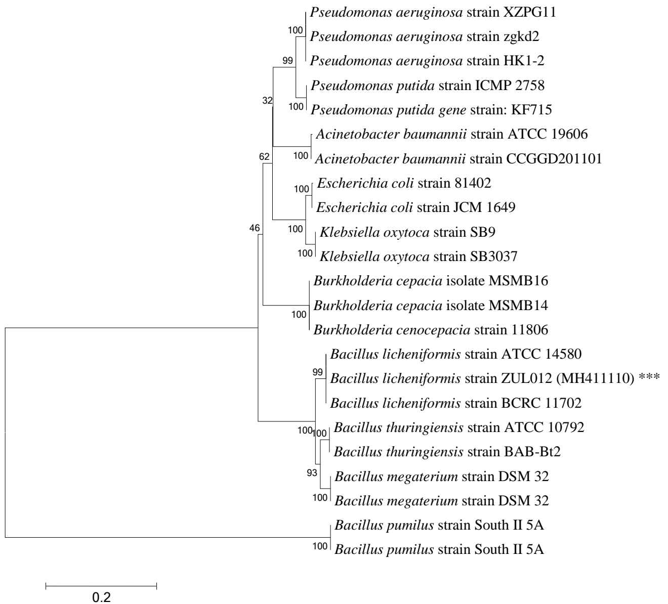
Fig. 1: Constructed Phylogenetic tree of the partial 16S rDNA sequences using Neighbor-Joining method. The scale bar corresponds to 0.2 changes per nucleotide. Numbers in parenthesis and asteriks represent GenBank accession numbers.
