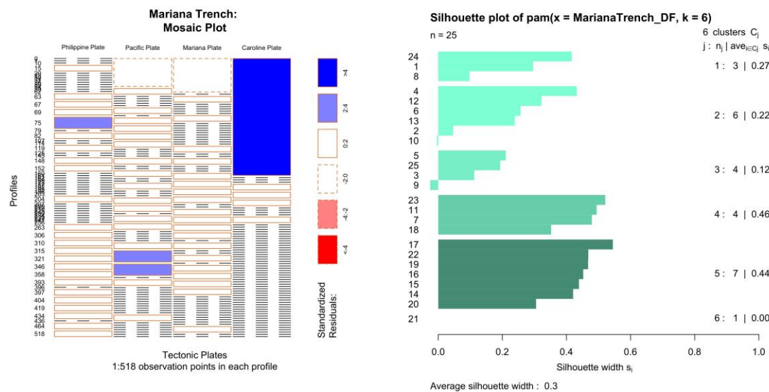
Figure 9. Mosaic plot and silhouette plots for categorical values of the environmental determinants of the Mariana Trench
