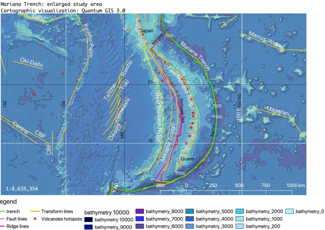
Figure 1. Study area: Mariana Trench. Cartography by QuantumGIS (QGIS)
