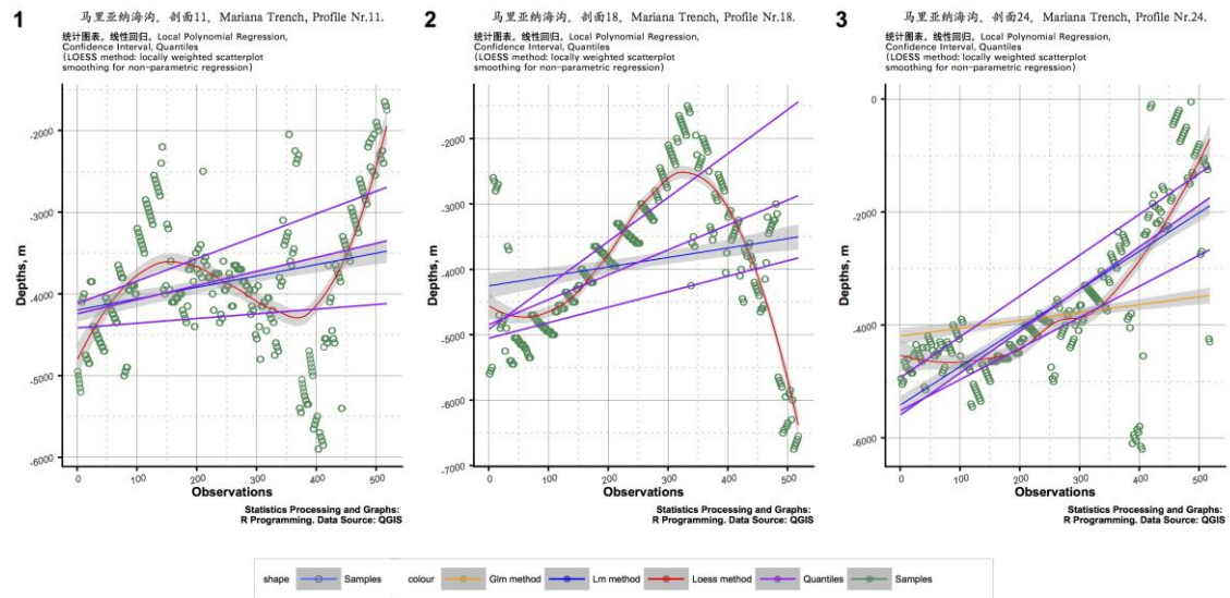
Figure 4. Regression analysis for selected profiles, R Programming
