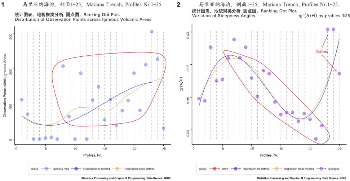
Figure 7. Ranking dot plots by data grouping
