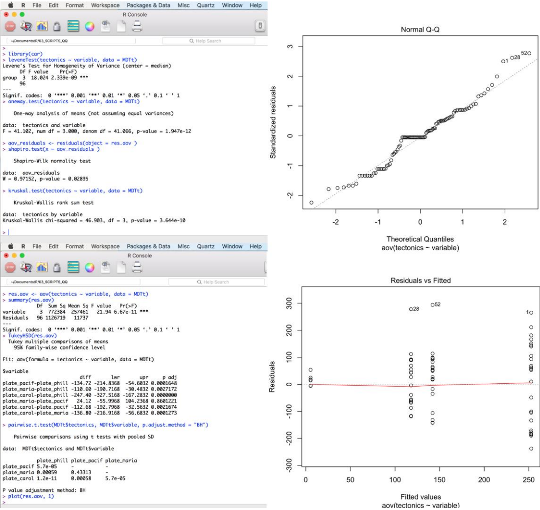
Figure 11. ANOVA hypothesis testing
