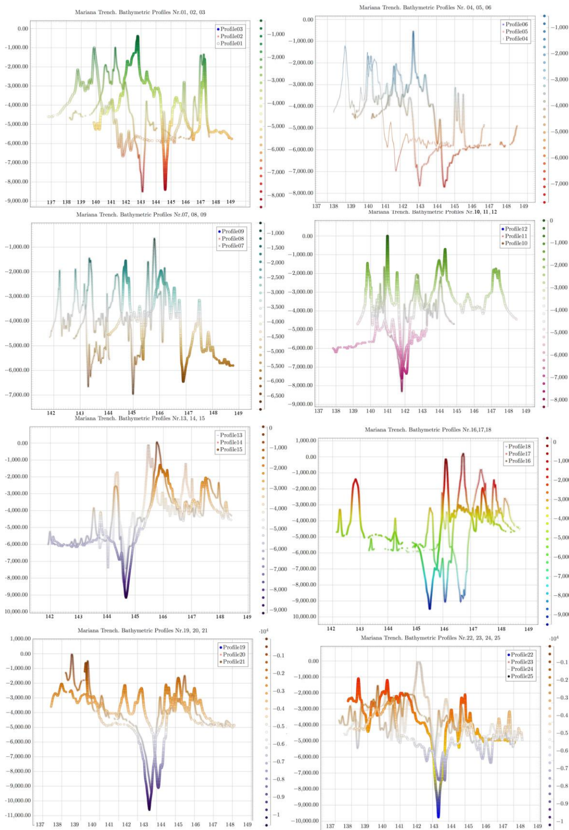
Figure 3. 25 cross-section bathymetric profiles of Mariana Trench. Plotting: LaTeX
