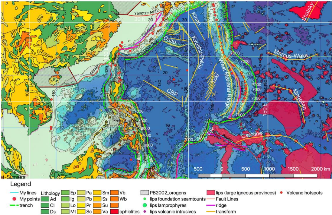
Figure 2. Lithology of the Mariana Trench area, Pacific Ocean. Map: QGIS
