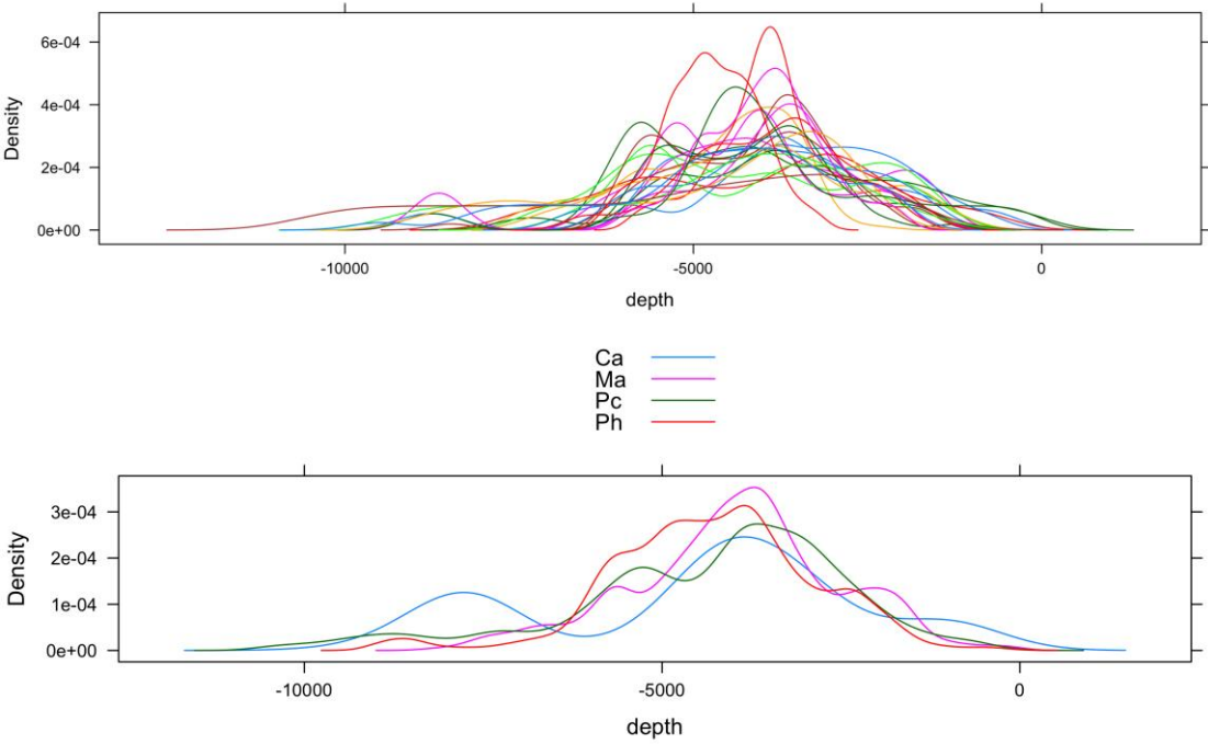
Figure 5. Kernel density estimation for 25 bathymetric profiles, Graph: R.
