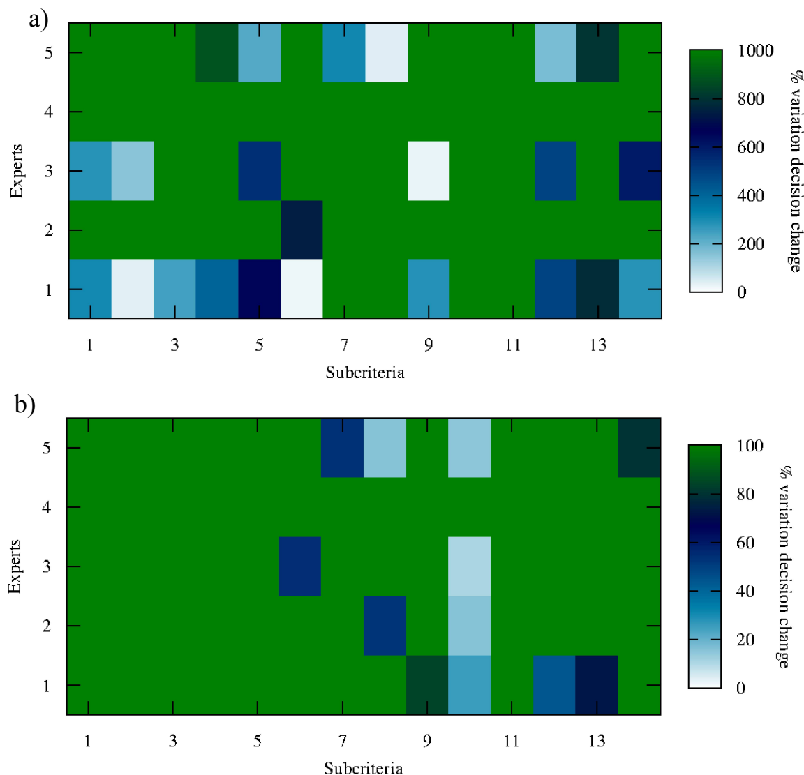
54 Figure S.I.A3. (a) Percentage variation of the individual sub-criteria weights at which the 55 ideal solution changes for the case of big scale distributed photovoltaic systems. (b) 56 Average of 1000 realizations of percentage variation of the individual sub-criteria together 57 with random errors in all the other sub-criteria of size equal or less than the percentage 58 variation in the considered sub-criteria. Each point shows the percentage at which the ideal 59 solution changes for the case of big scale distributed photovoltaic systems.
