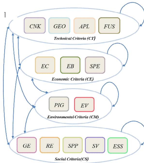
Figure S.I.A1. The interrelation among criteria, used for the evaluation of big scale systems. Notice that the arrows indicate that each cluster has relation with criteria within other clusters and within the same cluster.
