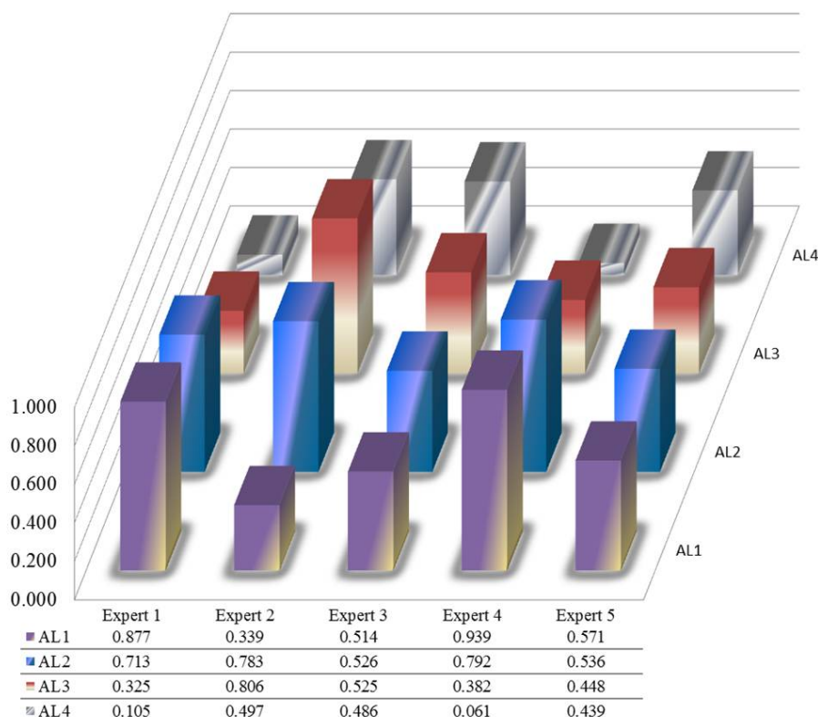
Figure S.I.A2. Relative proximity of each of the alternatives composing the size choices in large-scale distributed photovoltaic systems.
