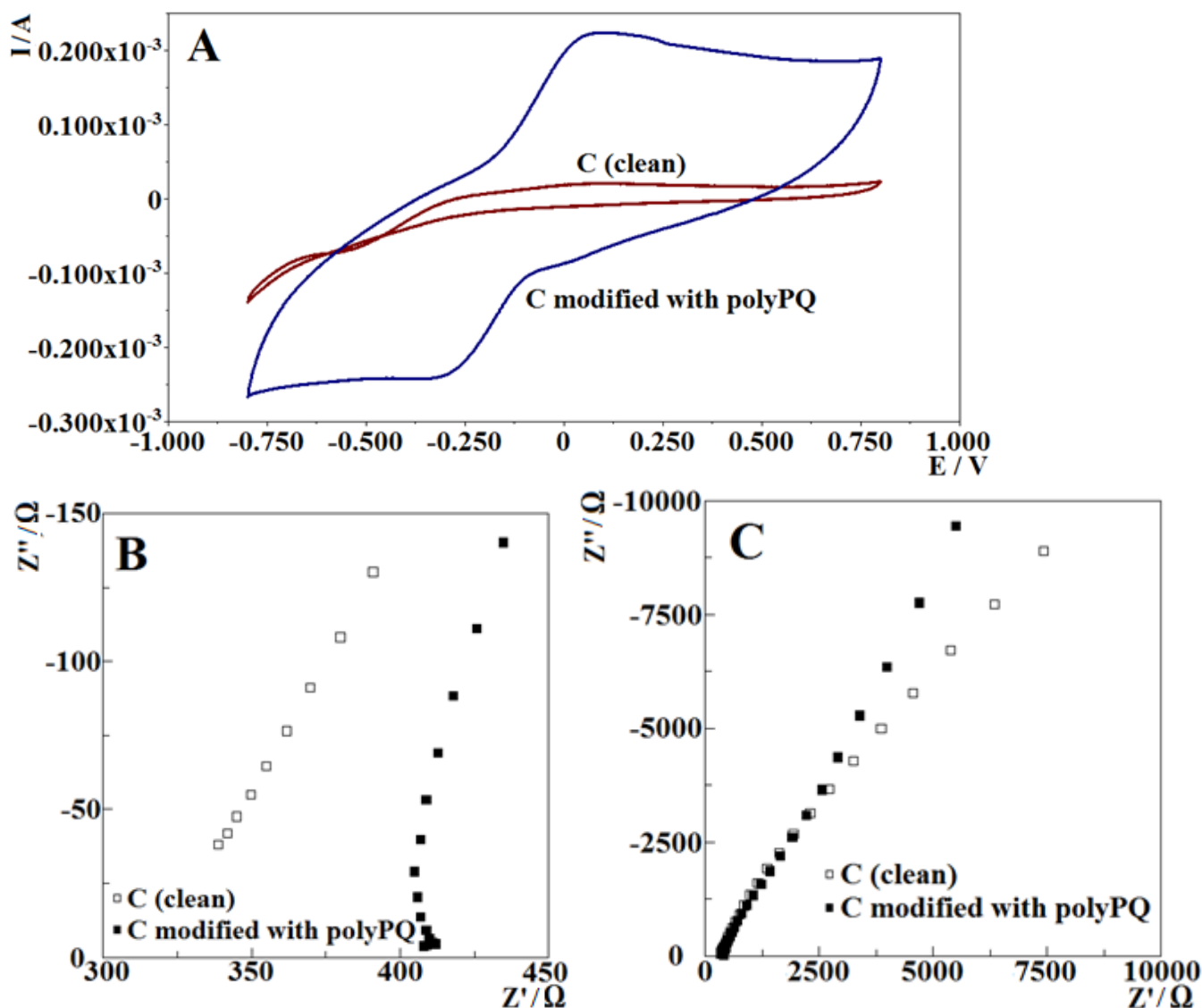
Fig. 6. A – Cyclic voltammograms of poly-PQ modified and unmodified GR electrodes in buffer solution; B – EIS spectra of poly-PQ modified and unmodified GR electrodes in high frequencies (40.0 kHz – 16.0 Hz) and C – in lower frequencies (16.0 Hz – 5.00 mHz) at 0 V vs Ag/AgCl/KCl (3M KCl) .
