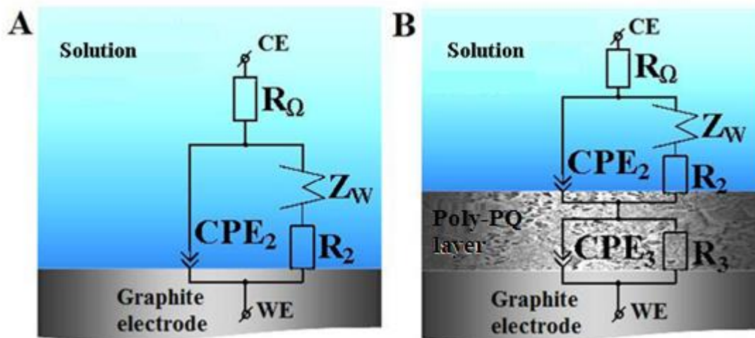
Fig. 3. Equivalent circuit for A– clean and B– poly-PQ coated graphite electrode.
