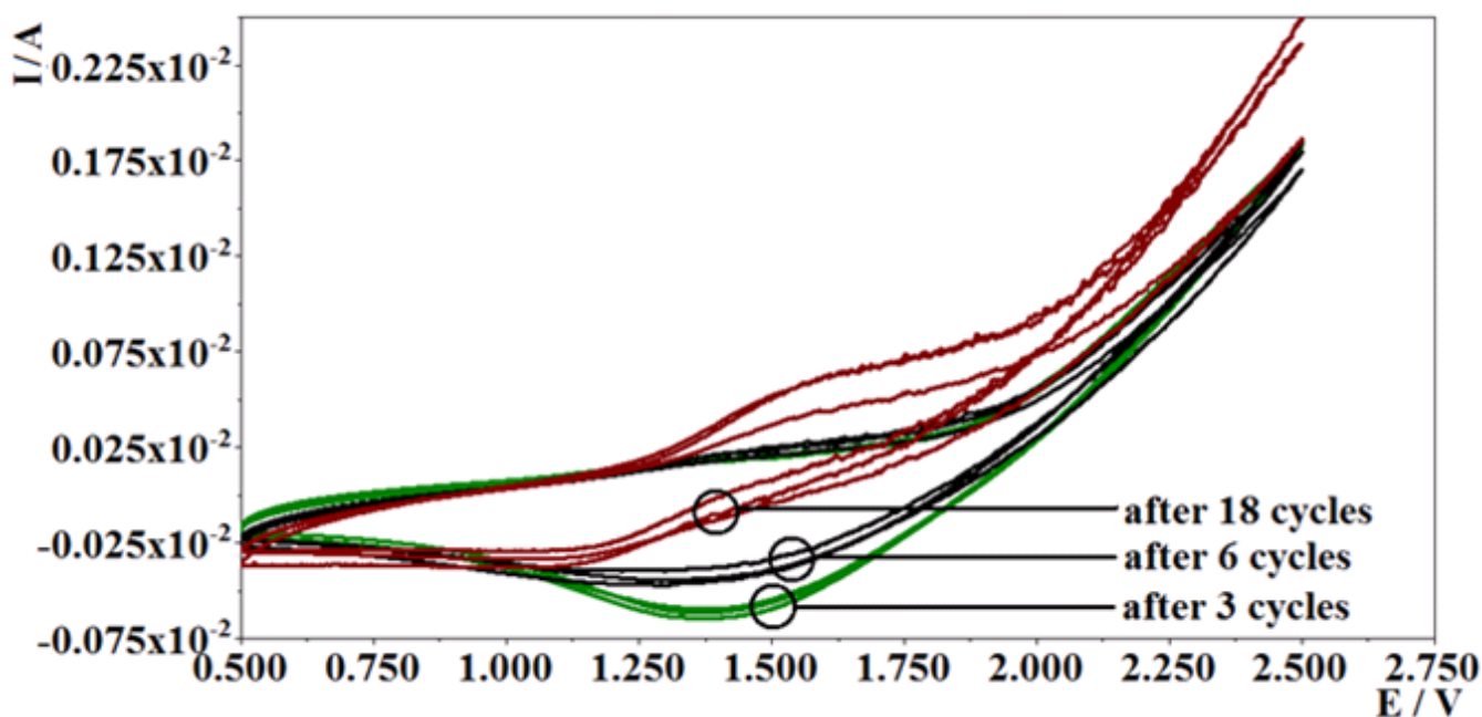
Fig. 1. Cyclic voltammograms obtained during potential cycling based polymerization of PQ.
