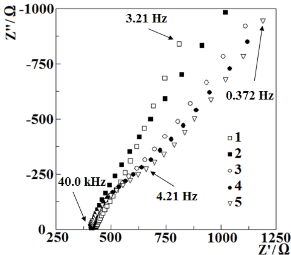
Fig. 2. EIS data gathered during the polymerization, 1 – recorded before polymerization, 2 – after 3, 3 – after 6, 4 – after 9 and 5 – after 18 polymerization cycles
