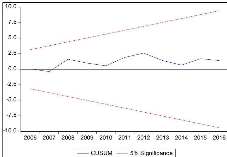
Figure 9. Plot of CUSUM.
