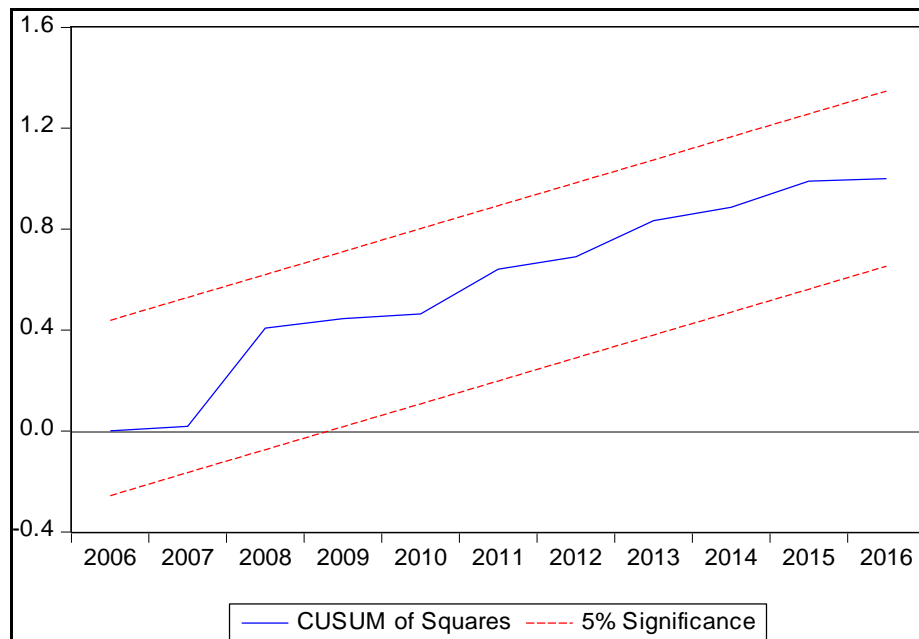
Figure 10. Plot of CUSUM of Square.
