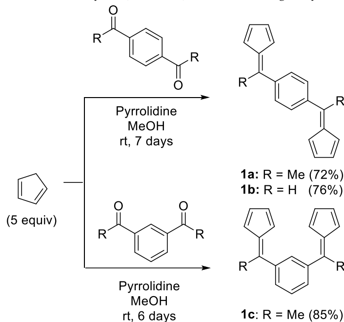
Scheme 2. Synthesis of para - and meta -phenylene-bridged bis(fulvenes) 1a–c .
