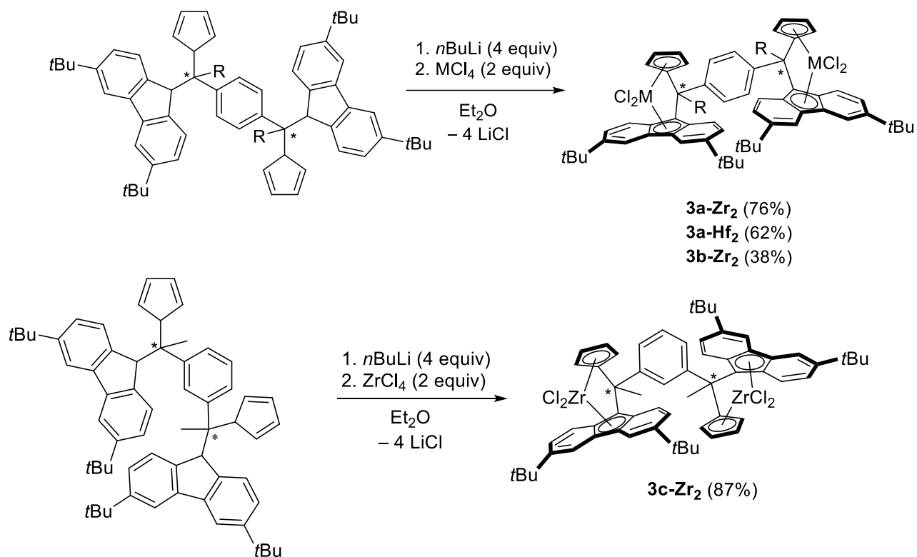
Scheme 4. Synthesis of group 4 homodinuclear bis(dichloro-ansa-metalloocene) complexes.
