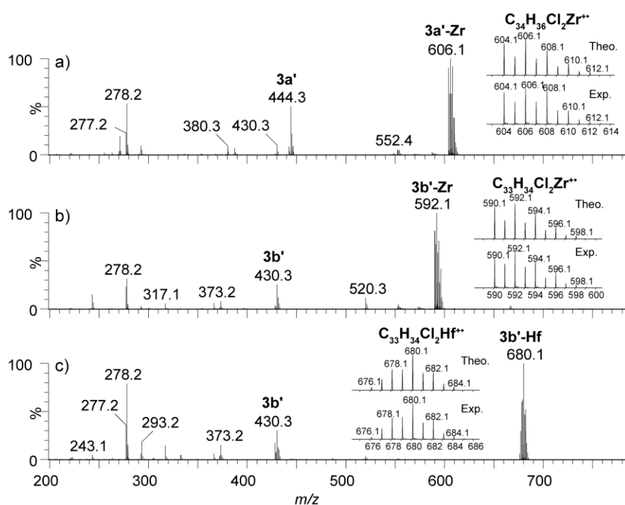
Figure 1. APPI(+) mass spectra of mononuclear complexes 3a'-Zr (a), 3b'-Zr (b) and 3b'-Hf (c). The zoomed areas showcase the theoretical and experimental isotopic clusters. For each isotopic distribution, only the most intense isotope peak is labelled.
