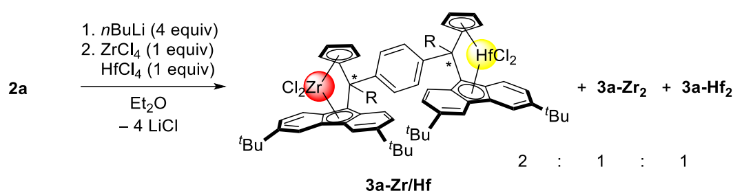
Scheme 6. Attempted synthesis of heterodinuclear bis(metallocene) 3a-Zr/Hf .
