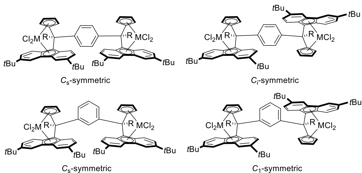
Scheme 4. Synthesis of group 4 homodinuclear bis(dichloro-ansa-metalloocene) complexes.
