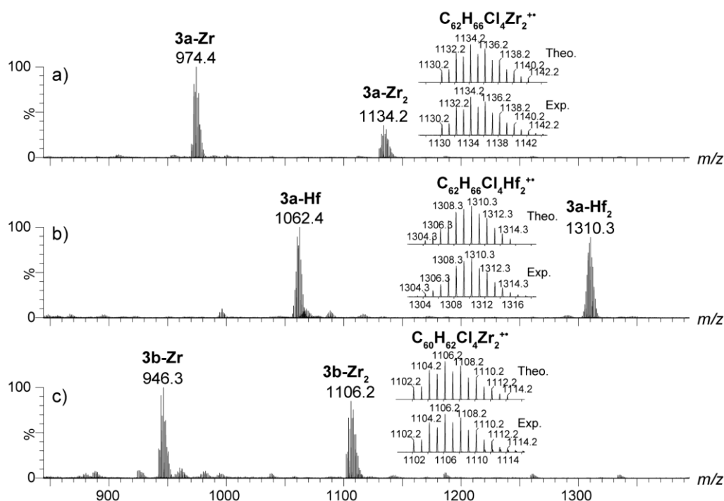
Figure 2. APPI(+) mass spectra of dinuclear bis(metalloocene) 3a-Zr 2 (a), 3a-Hf 2 (b) and 3b-Zr 2 (c) complexes. The zoomed areas showcase the theoretical and experimental isotopic clusters. For each isotopic distribution, only the most intense isotope peak is labelled.
