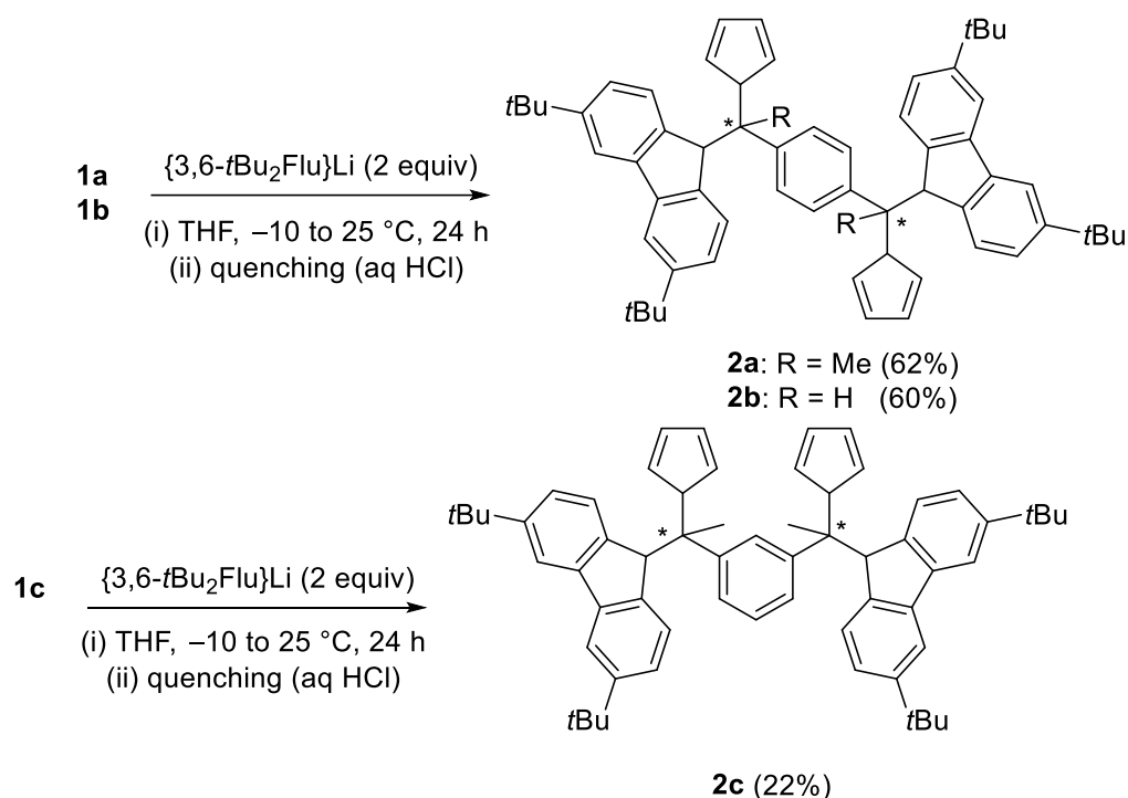
Scheme 3. Synthesis of proligands 2a–c .
