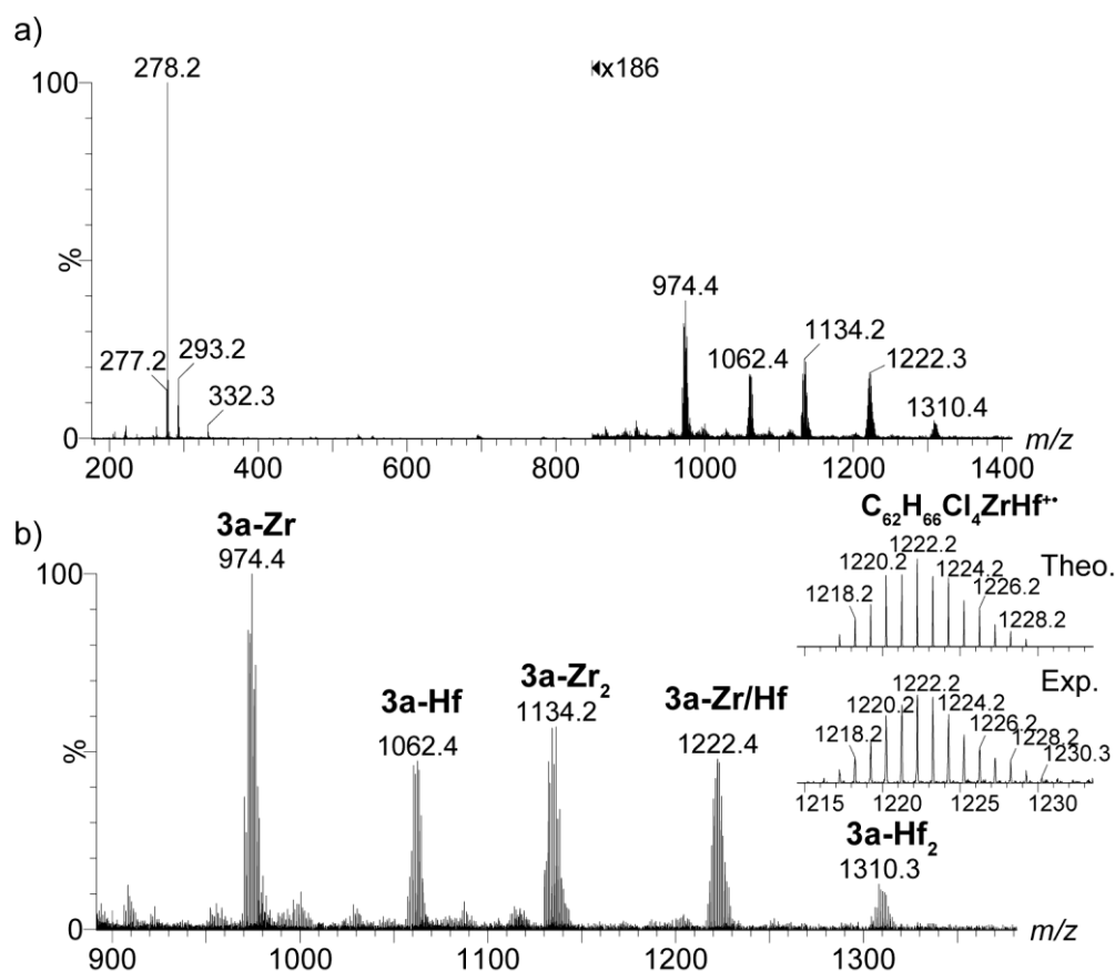
Figure 3. (a) APPI(+) mass spectrum of the crude reaction mixture resulting from metallation of proligand 3a by a 1:1 mixture of ZrCl_4 and HfCl_4 . (b) The enlargement of the m/z 900-1350 area. The zoomed areas showcase the theoretical and experimental isotopic clusters of dinuclear bis(dichloro ansa -metallocene) complexes 3a-Zr-Hf . For each isotopic distribution, only the most intense isotope peak is labelled.
