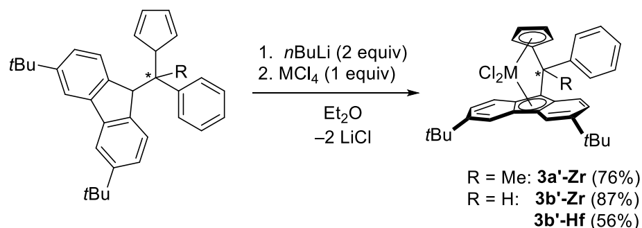
Scheme 7. Synthesis of mononuclear metallocene analogues.
