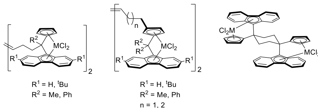
Scheme 1. Examples of group 4 dinuclear bis(dichloro ansa -metallocene) complexes incorporating \{R_2C(\text{Cp}/\text{Flu})\} ligand platforms.[8,9]
