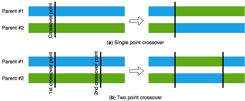
Figure 4. Genetic operator crossover between alleles. (a) Single point crossover in which one crossover point is selected, binary string from beginning of chromosome to the crossover point is copied from one parent, the rest is copied from the second parent. (b) Two point crossover in which two crossover point are selected, binary string from beginning of chromosome to the first crossover point is copied from one parent, the part from the first to the second crossover point is copied from the second parent and the rest is copied from the first parent.
