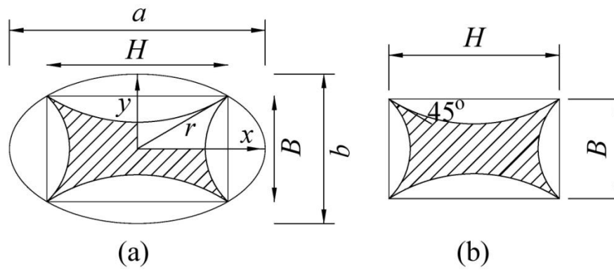
Figure 3. Effective confined concrete area in elliptical-sectioned column: (a) an elliptical jacketing scheme for an existing rectangular-sectioned column; (b) a rectangular concrete block with the same aspect ratio is considered, internal to the elliptical concrete section.
