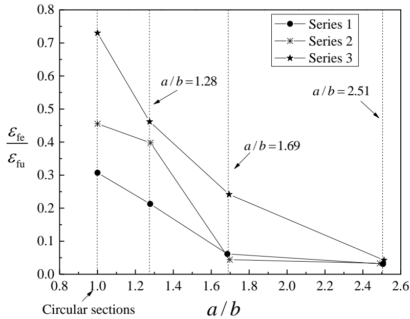
Figure 2. Effect of aspect ratio on FRP hoop strain: \varepsilon_{fe} = average FRP hoop strain from gauges on minor and major section sides; \varepsilon_{fu} = FRP tensile strain obtained from flat test coupons
