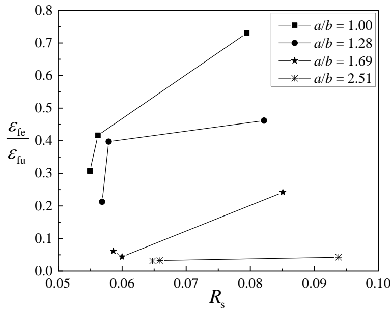
Figure 1. Effect of FRP confinement stiffness on hoop strain (Series 1 &5): \varepsilon_{fe} = average FRP hoop strain from gauges on minor and major section sides; \varepsilon_{fu} = FRP tensile strain obtained from flat test coupons
