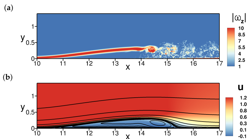
Figure 2. (a) Instantaneous spanwise-averaged spanwise vorticity. (b) Time and spanwise averaged streamline colored with u -velocity.
