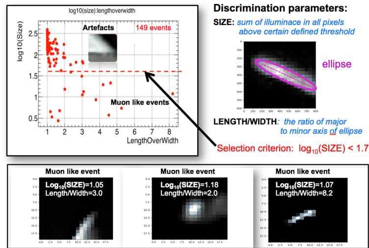
Figure 3. Example of classification of CREDO smartphone's images (see text for more details).
