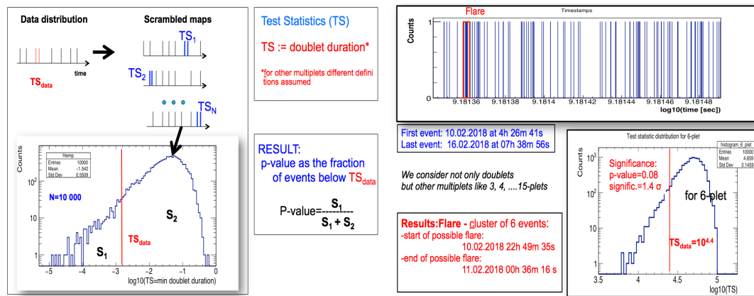
Figure 4. Left panel: Graphical explanation of time clustering algorithm, see text for more details. Right panel: Distribution of 100 detection timestamps from one smartphone corresponding to about 6 days of taking data with the CREDO Detector application. Some excess seems to appear at the beginning of the data acquisition i.e cluster of 6 events with significance of about 1.4 \sigma but this result is compatible with the background expectation.
