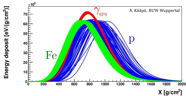
Figure 1. Longitudinal development of air showers induced by protons, iron nuclei and super-preshowers of primary energies E = 10^{19.6} eV, arriving at the Pierre Auger Observatory [8] from geographical South, at zenith angles of 60 deg [9].
