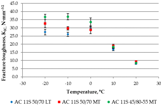
Figure 11. The results of fracture toughness from the Semi-Circular Bending Test (SCB)
