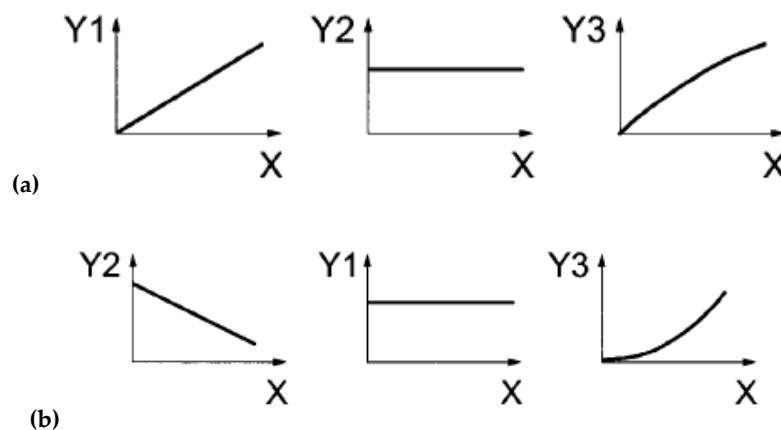
Figure 1. Test principles: a) Uniaxial Tension Stress Test (UTST), b) Thermal Stress Restrained Specimen Test (TSRST); where: X – time, Y1 – strain, Y2 – temperature, Y3 – stress, [11]
