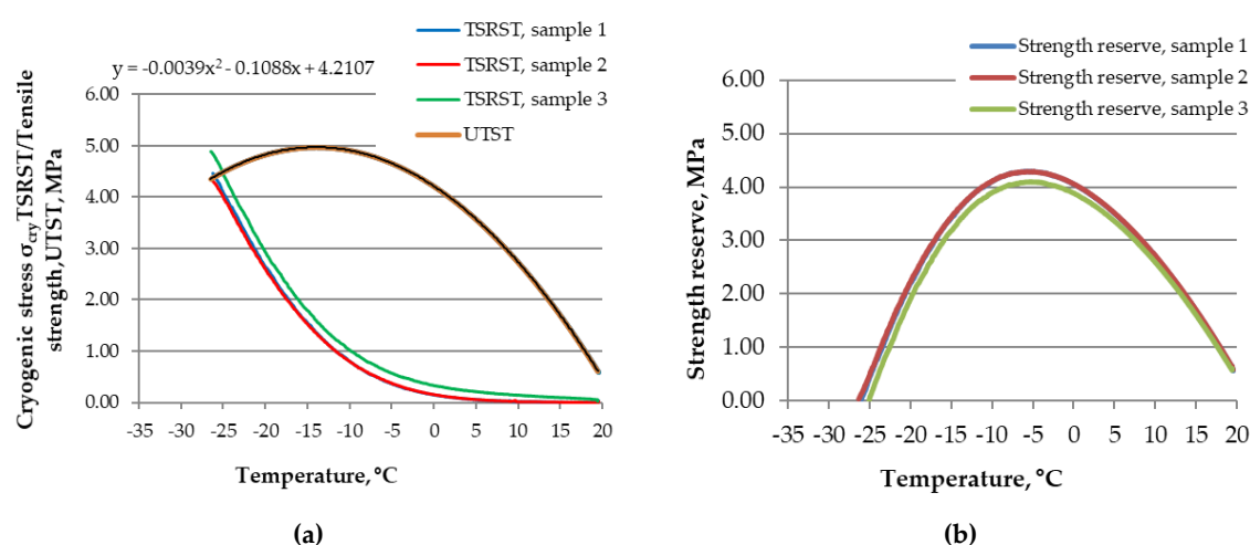
Figure 7. An example of the tensile strength reserve analysis, a) the TSRST and UTST results; b) graphical presentation of the tensile strength reserve results
