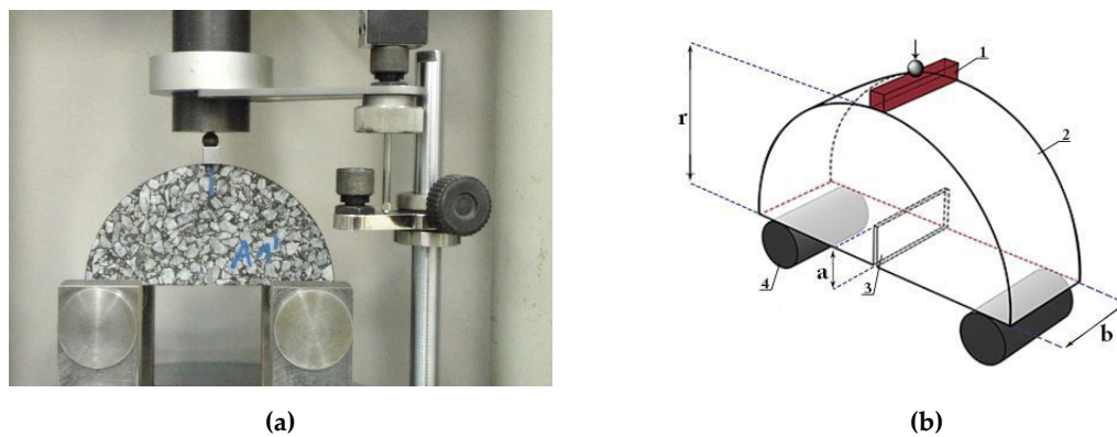
Figure 4. Semi-Circular Bending Test (SCB) with deflection strain rate setup: a) photograph of the test setup showing the specimen during the test, b) schematic view
