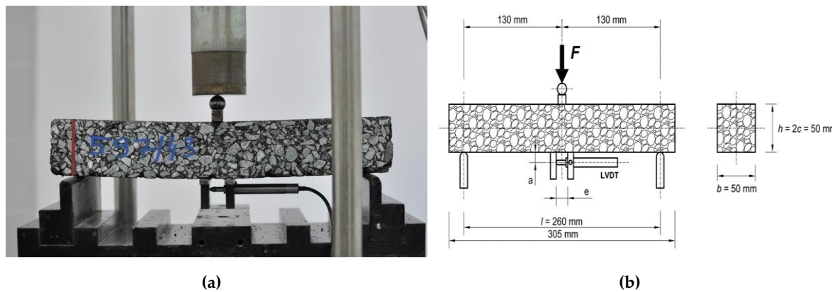
Figure 3. Bending Beam Test (BBT) with constant deflection rate setup: a) photograph of the test setup showing the specimen during the test, b) schematic view.
