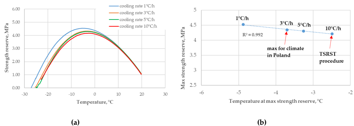
Figure 10. Influence of cooling rate on tensile strength reserve, a) strength reserve for different cooling rates, b) maximum strength reserve values versus temperature at the maximum strength reserve
