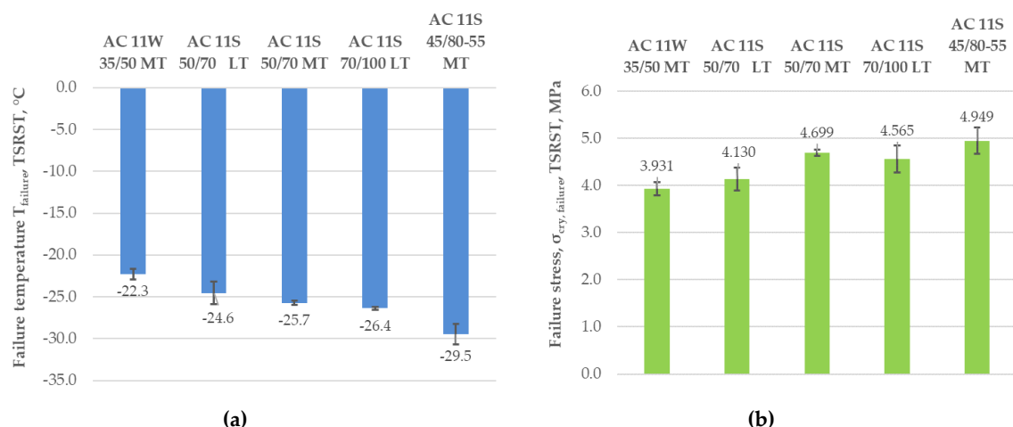
Figure 6. The results of failure temperature and failure stress from the Thermal Stress Restrained Specimen Test (TSRST), a) failure temperature T_{failure} , b) failure stress \sigma_{cry, failure}
