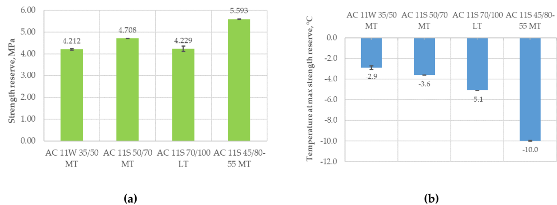
Figure 9. Influence of asphalt mixture and bitumen type on strength reserve results, a) maximum strength reserve results; b) temperature at the maximum value of strength reserve
