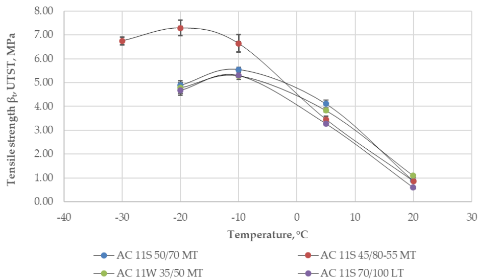
Figure 5. The results of tensile strength from the Uniaxial Tension Stress Test (UTST)
