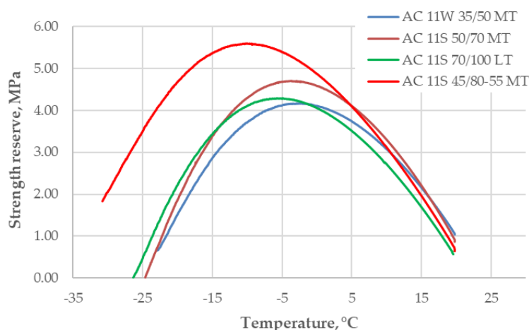
Figure 8. The results of strength reserve calculations
