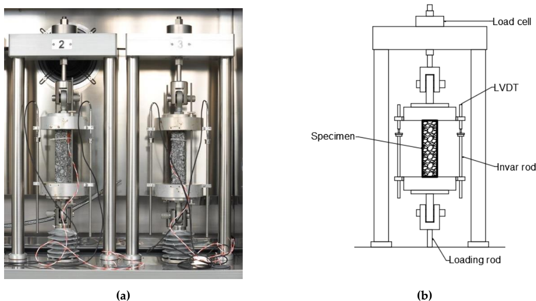
Figure 2. Uniaxial Tension Stress Test (UTST) and Thermal Stress Restrained Specimen Test (TSRST) setup: a) photograph of specimens during the test, b) schematic view.
