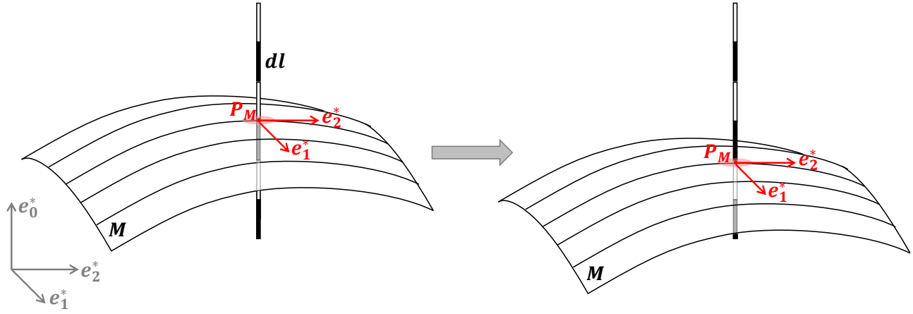
FIG. 2. Illustrative three-dimensional example: an infinitesimally thin rod in the \mathbf{e}_0^* direction, consisting of black and white elements of length dl . The flat observer at the point P_M in a submanifold M with basis \{\mathbf{e}_1^*, \mathbf{e}_2^*\} (red) measures the thin rod only as a point or very small disk. The observer can determine whether the disk is black or white. Now imagine the flat observer and the rod moving relative to each other along the \mathbf{e}_0^* direction (situation on the right). By counting the black and white elements that have passed through, the flat observer is given a measuring rule for distances which are not in his submanifold. In this example, the length of a black or white element serves as the standard length, the count corresponds to determining any distance as a multiple of the standard length. On the bottom left in grey the basis system \{\mathbf{e}_0^*, \mathbf{e}_1^*, \mathbf{e}_2^*\} of a local observer is shown, whose measurement is not limited to a submanifold.
