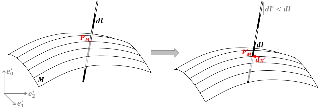
FIG. 3. Illustrative example: an infinitesimally thin rod tilted at a small angle from the \mathbf{e}_0^* direction. From the situation on the left to the situation on the right there is a relative displacement between the submanifold of the flat observer M and the rod. After defining the distance measurement outside of its submanifold M by counting black and white elements on the rod, the flat observer has to assume that the distance from black (situation on the left) to white (situation on the right) has remained the same as in Figure 2. In addition to this measuring rule, the total distance covered is given by ds'^2 = dl^2 + dx'^2 , which can be expected when using a mixed basis and choosing the length element \mathbf{e}^0 = d\mathbf{l} as the basis vector for lengths outside of M . In contrast, the local observer can use the basis vector \mathbf{e}_0^* as a reference and finds that the distance traveled in the \mathbf{e}_0^* direction is slightly shorter than the one in Figure 2 ( dl' < dl ). The local observer thus makes Euclidean measurements ds'^2 = dl'^2 + dx'^2 = dl^2 (indicated in gray).
