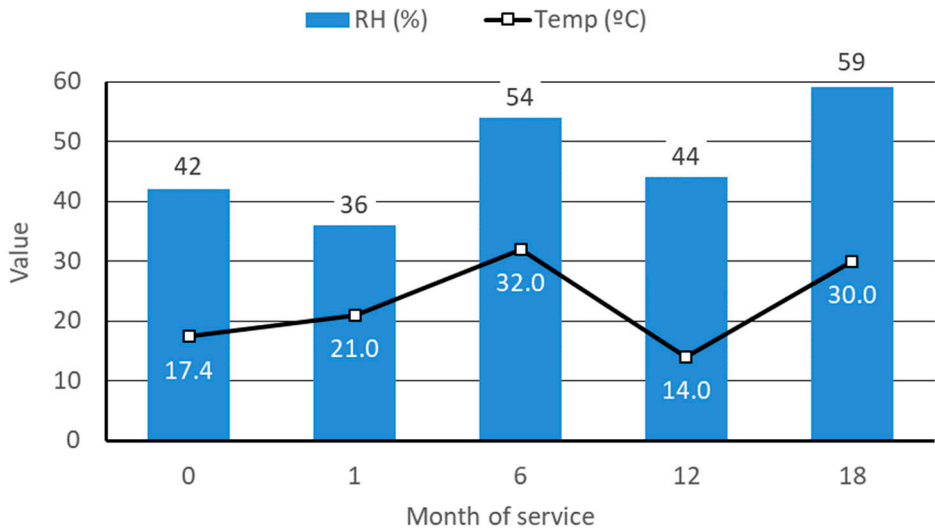
Figure 5. Surface temperature and relative humidity measured in the test section during data collection.
