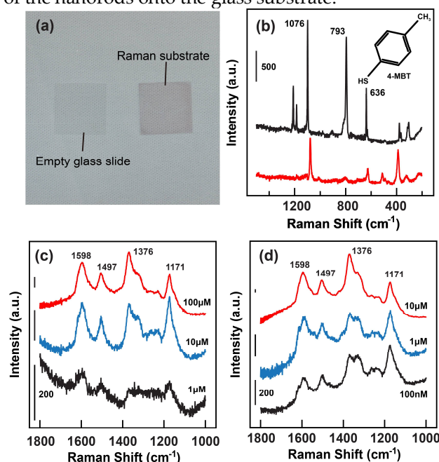
Figure 3. SERS activity of the large-aspect-ratio gold nanorods. (a) Digital photograph of the SERS substrate fabricated with glass slide. (b) Raman spectra of the 4-MBT on the SERS substrate (red) and in powder form (black). The molecular formula of the 4-MBT is presented in the inset. The spectrum of the molecular powder was collected using a laser power of 118.00 mW, while that from the SERS substrate was collected with a
