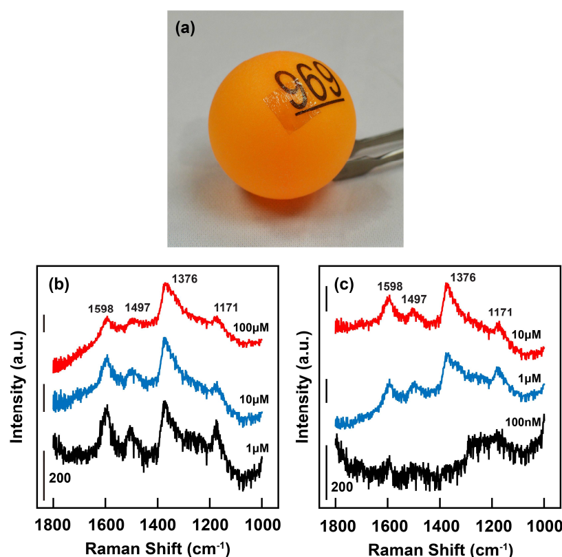
Figure 4. Flexible SERS substrate. (a) Digital photograph of the flexible SERS substrate stuck onto the surface of a table tennis ball; (b) Raman spectra of the PANI-ES molecules of different concentrations collected from the empty PS substrate; (c) Raman spectra of the PANI-ES molecules of different concentrations collected from the flexible SERS substrate. The excitation wavelength for (b) and (c) is 1064 nm. The baselines of the Raman spectra have been modified for better demonstration.
