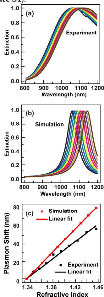
Figure 2. Refractive index sensitivity of the gold nanorods with large aspect ratios. (a) Extinction spectra of the gold nanorods stabilized in glycerol–water mixture with varied glycerol volume ratios. (b) Simulated extinction spectra of the gold nanorod immersed in media with varied refractive indexes. (c) Dependence of the longitudinal plasmon shift on the refractive index of the liquid mixture for the gold nanorods. Black and red symbols are experimental and simulated results, respectively. The lines are linear fits.
