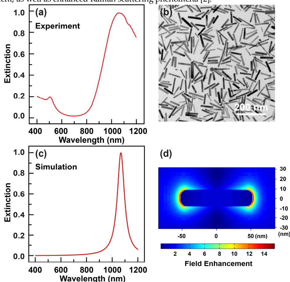
Figure 1. Characterizations of the gold nanorods of large aspect ratios. (a) Experimental extinction spectrum of the gold nanorod aqueous solution. (b) TEM image of a typical gold nanorod sample. (c) Calculated extinction spectrum of an individual gold nanorod. The geometrical parameters of the nanorod are set according to those measured from the image shown in (b). (d) Calculated near-field electromagnetic distributions around the individual gold nanorod. The electric fields are monitored at the extinction maximum shown in (c), and on the plane across the longitudinal axis of the nanorod.
