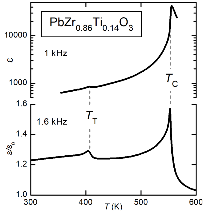
Figure 3. Compliance and dielectric permittivity of \text{PbZr}_{0.86}\text{Ti}_{0.14}\text{O}_3 , with anomalies at T_C and the octahedral tilting transition at T_T (data from Ref. [29])
