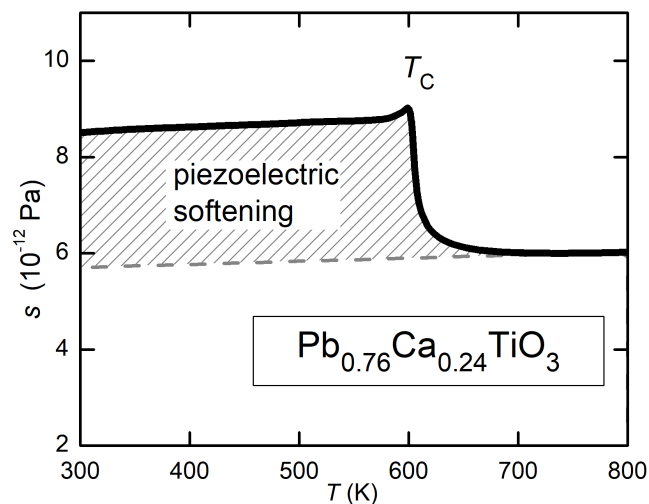
Figure 5. Preliminary measurement of the compliance of a sample of (\text{Pb,Ca})\text{TiO}_3 .
