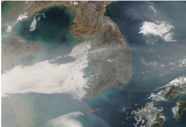
Figure 1. NASA satellite image shows a swath of air pollution sweeping east across the Korean peninsula to Japan [24]
