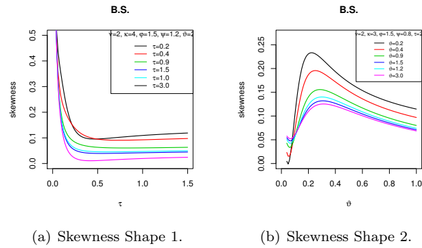
Figure 8: Plot of the BKBX Skewness for different parameter values of \nu, \kappa, \varphi, \psi and \tau .
