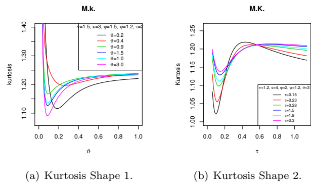
Figure 9: Plot of the BKBX Kurtosis for different parameter values of \nu, \kappa, \varphi, \psi and \tau .
