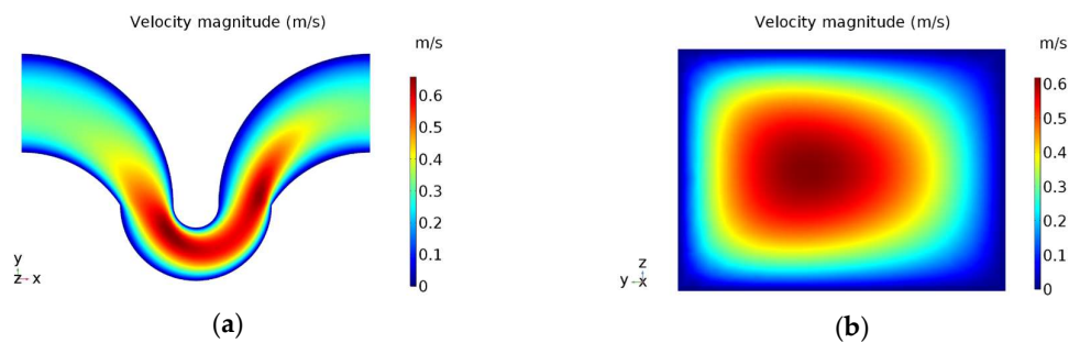
Figure 6. (a) Flow velocity magnitude for Q=130 \mu\text{L}/\text{min} and h=73 \mu\text{m} measured at z=36.5 \mu\text{m} , at the middle height of the fluidic channel; (b) Flow velocity magnitude for the same flow conditions measured at the y-z plane halfway through the small curve.
