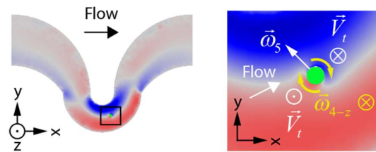
Figure 13. Left: z -component of the lateral flow field. Reddish regions correspond to flow moving upwards and vice versa for bluish regions. Right: The vertical rotational component of the particle ( \omega_{4-z} ) induces a disturbance in this component of the lateral flow field (yellow arrows) that modifies the behavior of the rotating particle ( \omega_5 component).
