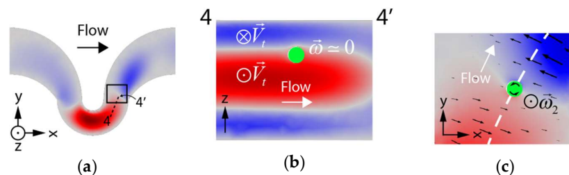
Figure 14. Transverse velocity magnitude and sense of the flow. (a) General view of the channel with marked cross sections; (b) The interface between the outwards and inwards-moving flow is no longer distorted so no modification of the angular velocity vector is produced in this region; (c) A strong induced angular velocity ( \omega_2 , with positive z direction) is observed at the vicinity of the transverse inwards-outwards transition region.
