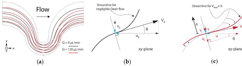
Figure 3. (a) Obtained streamlines for a flow with negligible Dean flow (black lines) and for Q=130 \mu\text{L}/\text{min} (red lines) for h=73 \mu\text{m} measured at z=36.5 \mu\text{m} . Dean flows at this height displace the streamlines outwards in the central region of the curves; (b) Decomposition, at any given point, of a flow velocity vector ( \vec{v} ) to a direction perpendicular to its corresponding negligible Dean flow streamline at that point. The perpendicular direction ( \hat{n} ) is found using the variables u_0 and v_0 from the solution at low flow rates; (c) Once the flow rate is increased, Dean flow appears and the velocity vector, now with v and u components, can be projected along vector \hat{n} .
