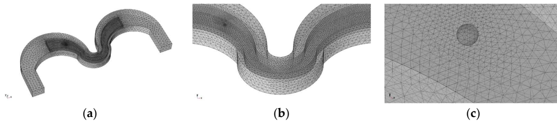
Figure 4. (a) Meshed simulation domain for the FSI simulation. The fluid enters the domain through one of the straight section ends; (b) Detail of the different sized meshes. The upper one corresponds to the region of the domain where the particle will translate through the curve; (c) Zoomed section of the mesh showing the particle domain at its initial position inside the channel.
