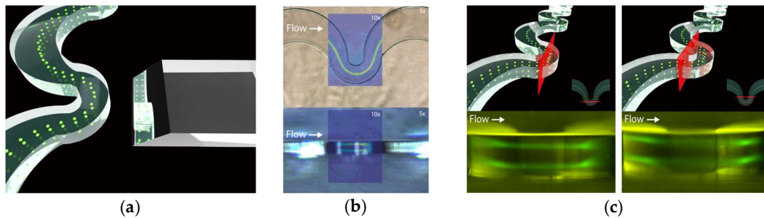
Figure 1. (a) Render that illustrates the position of the lateral mirror with respect the serpentine; (b) Zenithal (top) and lateral (bottom) views of the serpentine with an overlapped fluorescence streak image (false color) from inertially focused particles; (c) The limited depth of field of the employed objective allows to focus the streak of particles reflected in the mirror at different focus planes (red planes).
