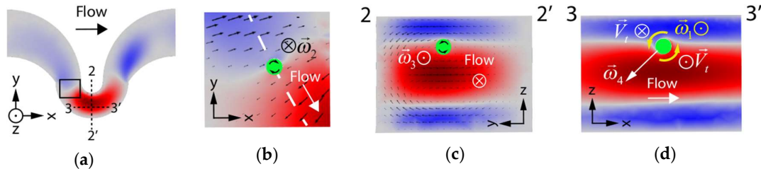
Figure 12. Simulated transverse velocity magnitude and sense of the flow. Reddish regions correspond to outwards-moving flow (moving away from the center of curvature of the small curve) and vice versa for the bluish regions. (a) General view of the channel with marked cross sections; (b) Transverse flow field gradients in the x-y plane induce particle's rotation, \omega_2 ; (c) The flow around the particle in the center of the Dean vortex further induces a change in the particle's rotation with a \omega_3 component in the x direction; (d) The rotating particle causes a disturbance (yellow arrows) at the interface between outwards and inwards lateral flows with V_t components which in turn causes a modification in the angular velocity of the particle yielding to \omega_4 component.
