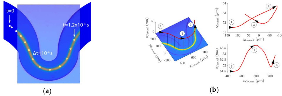
Figure 9. (a) Overlapping of the experimental image for a focused streak of \phi = 10 \mu m particles and positions of the particle calculated with the FSI simulation along the small (white circles). The overlapped image is represented in false color to improve the visibility of the streak; (b) Composed perspective of the 3D trajectory of particle (red line).
