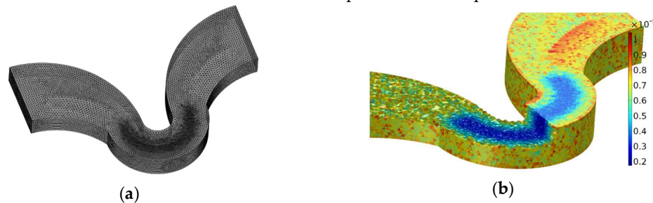
Figure 2. (a) Meshed simulation domain for the CFD simulation represented as a periodic unit of the serpentine. The channel is 73 \mu\text{m} in height; (b) Inner region of the simulation domain. Part of the mesh has been removed to expose the insides of the mesh emphasizing the effects of the finer mesh regions in the small curve. Color scale (in microns) represents the mesh element size.
