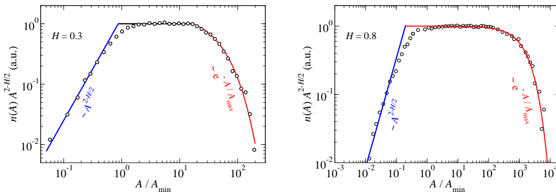
Figure 5. Distribution of contact-patch sizes n(A) divided by the scaling law n(A) \propto A^{2-H/2} at a reduced pressure of p_0^* = 0.04 . Left: H = 0.3 , right H = 0.8 . System specification: \mathcal{L}/\lambda_r = 4 , \lambda_r/\lambda_s = 512 .
