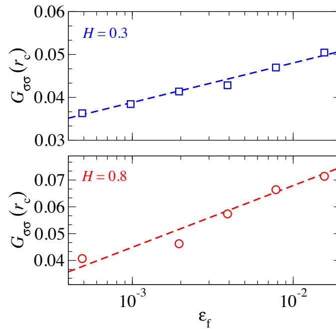
Figure 9. Value of the stress ACF, G_{\sigma\sigma}(r_c) , at the characteristic contact radius r_c \equiv \sqrt{A_c/\pi} for various values of \epsilon_f . System specification: \mathcal{L}/\lambda_r = 1 , p^* = 0.04 .
