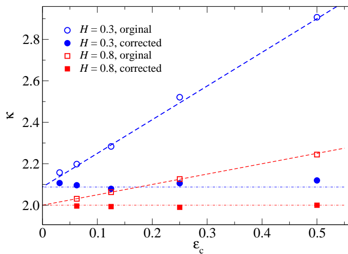
Figure 1. The dimensionless coefficient \kappa as a function of the discretization obtained with and without continuum corrections for H = 0.3 and H = 0.8 . A value of c = 1/8 was used in Eq. (6) for the corrected contact area. \kappa \equiv a_r/p_0^* , where p_0^* \equiv p_0/E^* \bar{g} is the reduced pressure. System specification: \mathcal{L}/\lambda_r = 1 , \lambda_r/\lambda_s = 256 , p^* = 0.04 .
