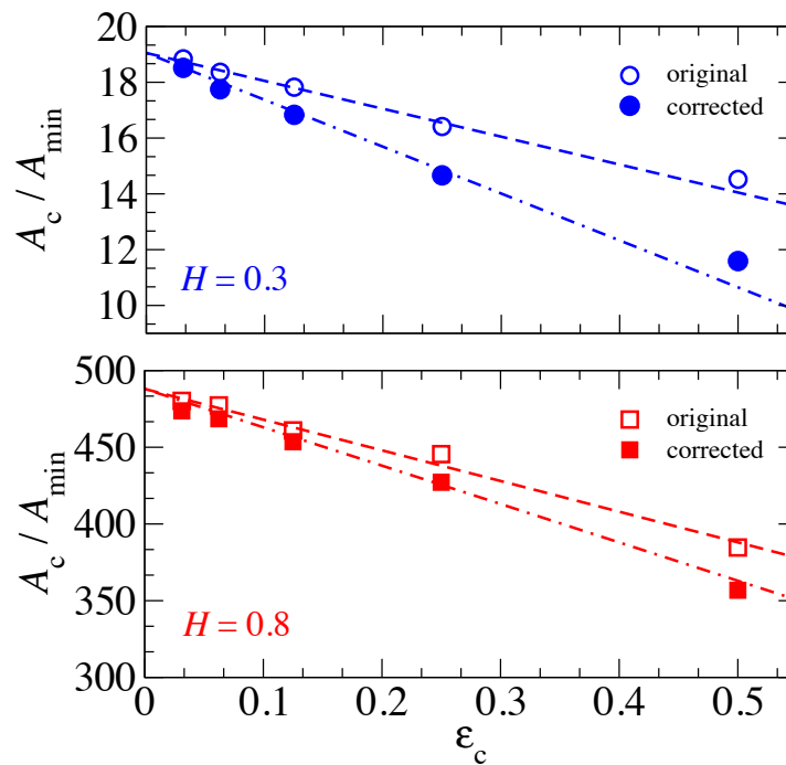
Figure 2. Characteristic contact area with and without continuum corrections as a function of \varepsilon_c = a/\lambda_s . System specifications: \mathcal{L}/\lambda_r = 1 , \lambda_r/\lambda_s = 512 , p_0^* = 0.04 .
