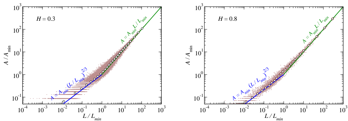
Figure 4. Individual patch size A_n versus load carried by each patch L_n (dots). Left: H = 0.3 , right H = 0.8 . Stripes in the scatter plot result from space discretization at small A . The open circles indicate running averages of the numerical data. Solid lines represents the theoretical prediction. System specifications: \mathcal{L}/\lambda_r = 4 , \lambda_r/\lambda_s = 128 , p^* = 0.04 .
