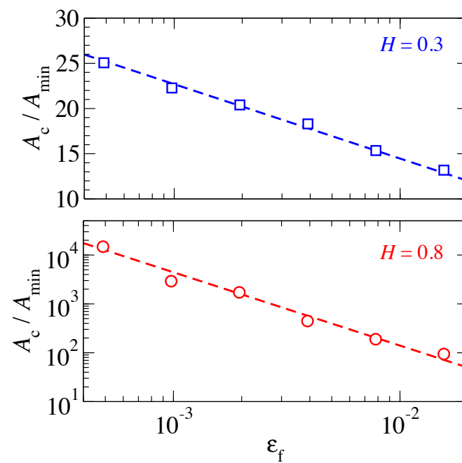
Figure 7. Characteristic contact-patch size as a function of the ratio \varepsilon_f = \lambda_s / \lambda_r at a fixed load for a H = 0.3 (top) and for a H = 0.8 (bottom) surface. The dashed lines are drawn to guide the eye. For the H = 0.8 , the dashed line reflects an \varepsilon_f^{-1.5} power law. Note that the ordinate is linear for H = 0.3 but logarithmic for H = 0.8 . System specification: \mathcal{L} / \lambda_r = 1 , p^* = 0.04 .
