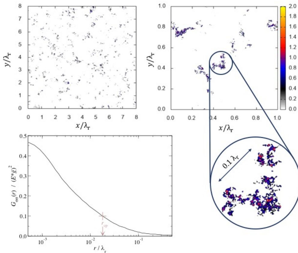
Figure 3. Top left, top right, and bottom right: Visualization of contact stresses in a randomly rough contact at different magnifications. Stresses in the color bar are given in units of E^* \bar{g} . Lower left: Stress autocorrelation function. System specification: \mathcal{L}/\lambda_r = 8 , \lambda_r/\lambda_s = 250 , p_0 = 0.01 E^*/\bar{g} , leading to a relative contact area of a_r \approx 0.02 .
