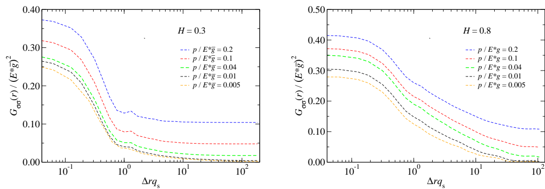
Figure 10. Stress ACF as a function of distance r at selected values of the reduced pressure p^* = p/E^*\bar{g} for H = 0.3 (left) and H = 0.8 (right). System specification in both cases: \mathcal{L}/\lambda_r = 4 and \lambda_r/\lambda_s = 512 .
