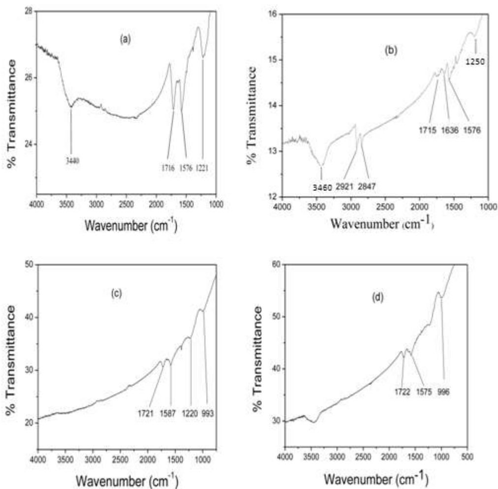
Fig.2. FTIR data for (a) MWCNT-COOH, (b) MWCNT-ODA, (c) p-MWCNT-Pd and (d) np-MWCNT-Pd
