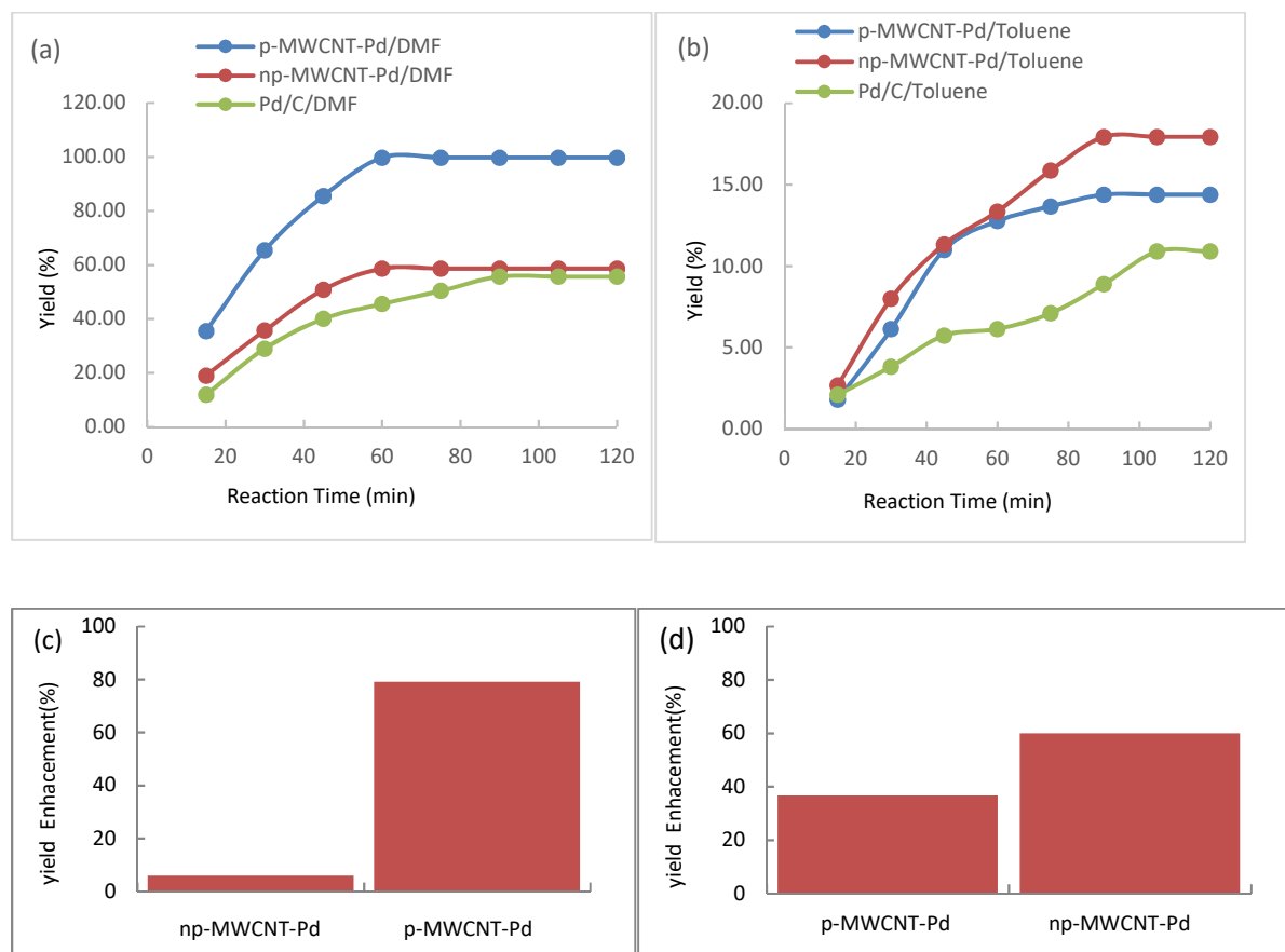
Fig.6. Yields of the CNT-metal nanohybrids and Pd/C catalyzed reactions (a) in DMF and (b) in toluene from GC analysis (Tri-butyl amine as base, temp 150°C); (c) yield enhancement with respect to Pd/C in DMF; (d) enhancement with respect to Pd/C in toluene
