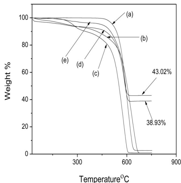
Fig.3. TGA of (a) MWCNT, (b) MWCNT-COOH, (c) MWCNT-ODA, (d) p-MWCNT-Pd and (e) np-MWCNT-Pd
