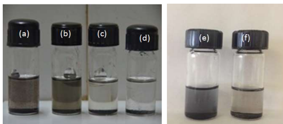
Fig.4-1 Photographs of different dispersions: (a) np-MWCNT-Pd dispersed in DMF, (b) p-MWCNT-Pd dispersed in DMF, (c) np-MWCNT-Pd in Toluene, (d) p-MWCNT-Pd in Toluene; Fig.4-2 (e) Pd/C dispersed in DMF, (f) Pd/C dispersed in Toluene.
