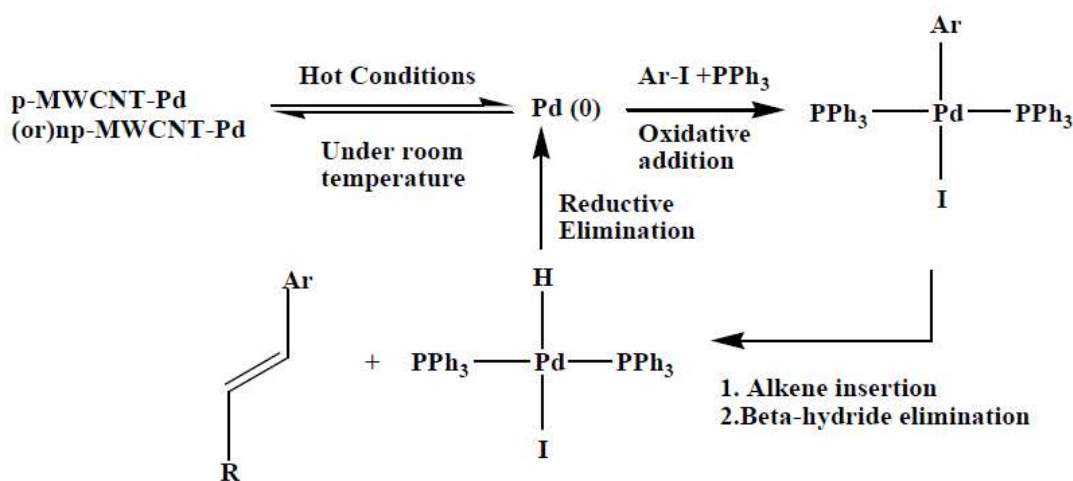
Fig.5. The role of CNT-Pd in the in Heck reaction
