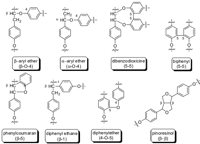
Figure 3. Structure of the three monolignol precursors and their corresponding fragments in the macromolecules.
