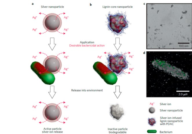
Figure 7 Schematics of the general use cycle and principle of the bactericidal action of environmentally benign lignin-core nanoparticles (EbNPs) and the currently used silver nanoparticles (AgNPs). a , General mechanism for the antimicrobial action of common AgNPs via the release of Ag + ions, which continues post-utilization. b , Mechanism of antimicrobial action of Ag + ion-infused EbNPs with a cationic polyelectrolyte coating that facilitates electrostatic attraction between the EbNPs and negatively charged cell walls. In contrast to AgNPs, EbNPs are depleted of Ag + ions during their application, minimizing their post-utilization activity. c , TEM micrograph of as-synthesized EbNPs in the size range of 40–70 nm. d , Confocal microscopy image of EbNPs with polyelectrolyte coating adhering to the cell membrane of E. coli .
