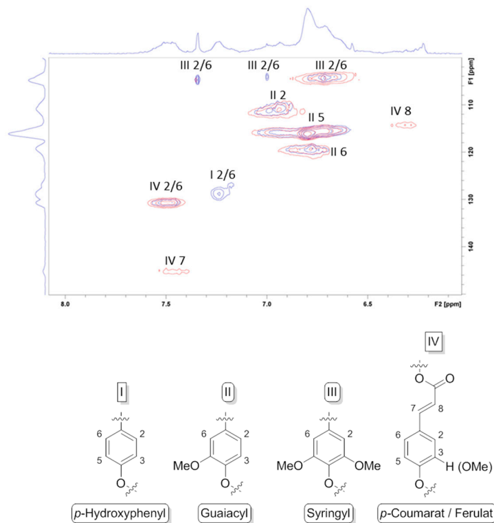
Figure 5. HSQC NMR spectrum, aromatic region (dC/dH 100–150/6.0–8.0) of lignin samples obtained via Organosolv process from Miscanthus X giganteus . Comparison of leaf lignin (blue) and stem lignin (red) and corresponding assigned lignin fragments. Copyright Springer 2018.
