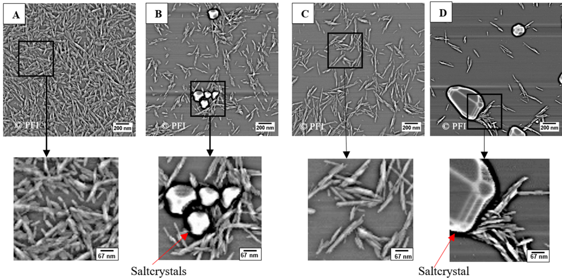
Figure 8. Image A and B is 0.02 wt % CNC (USDA) in deionized water and 0.1 wt % NaCl, while image C and D is 0.02 wt % CNC (AITF) in DIW and 0.1 wt % NaCl, respectively. The round shapes in image B and D are salt crystals. For all the images a small section has been enlarged three times to make it easier to see the fibrils and salt crystals in more detail.
