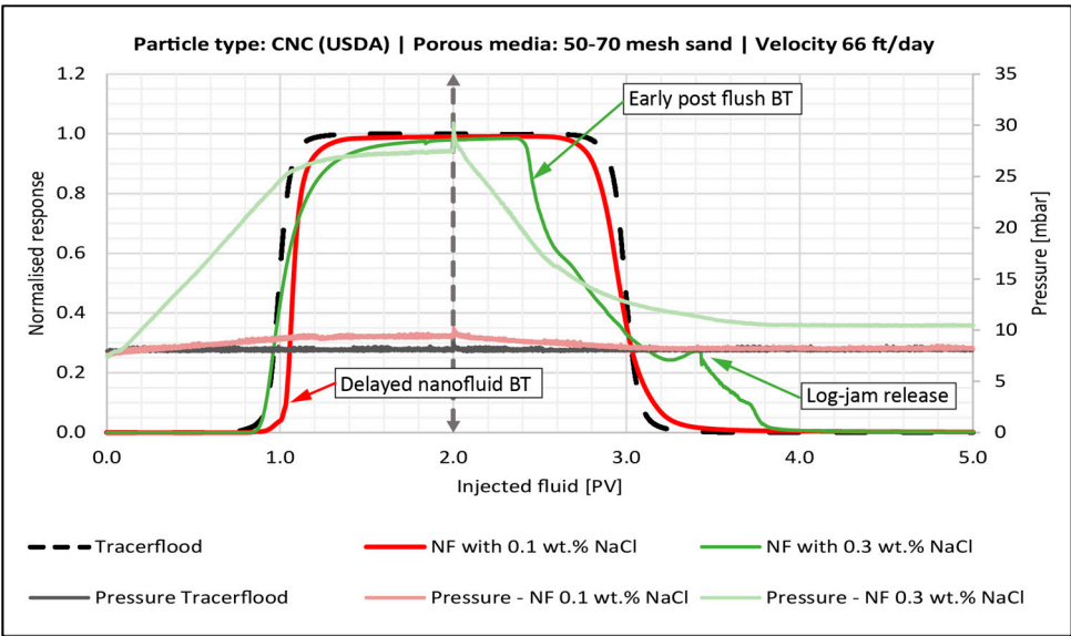
Figure 12. Breakthrough curve for the sandpackflood with 0.5 wt % CNC (USDA) in 0.1 wt % NaCl (red line) and 0.3 wt % NaCl (green line). Dashed vertical line illustrates the switch to post flush fluid. The tracer BT-curve is the black dotted line. The corresponding pressure curves are also shown.
