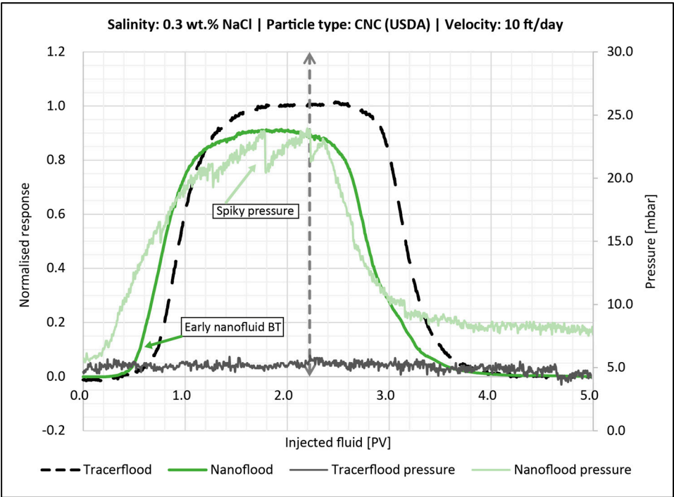
Figure 17. Breakthrough curve for the core flood with 0.5 wt % CNC (USDA) in 0.3 wt % NaCl (green line). 2.2 PV were injected followed by 0.3 wt % brine. The dashed vertical line illustrates when post flush was started. The tracer BT-curve is the black dotted line. The corresponding pressure curves are also shown.
