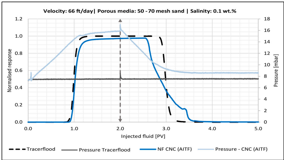
Figure 11. Breakthrough curve for the sandpack flood with 0.5 wt % CNC (AITF) (dark blue line) using a medium velocity (66 ft/day). Dashed vertical line illustrates the switch to post flush fluid. The tracer BT-curve is the black dotted line. The corresponding pressure curves are also shown.
