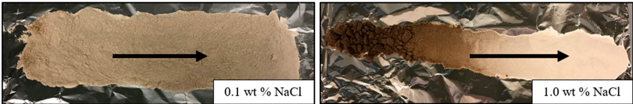
Figure 14. Evidence of nanocellulose retention from post-flood sand baking. Darkness correlates with mass of nanocellulose retained in sand after post flush. Arrows indicate flow direction in original sandpack. (Left) 0.5 wt % CNC (USDA) in 0.1 wt % NaCl at 66 ft/day resulted in uniformly distributed retention. (Right) 0.5 wt % CNC (USDA) in 1.0 wt % NaCl at 66 ft/day resulted in large retention near inlet decreasing to little or no retention in the downstream half of the sandpack. Both using 50-70 mesh sand.
