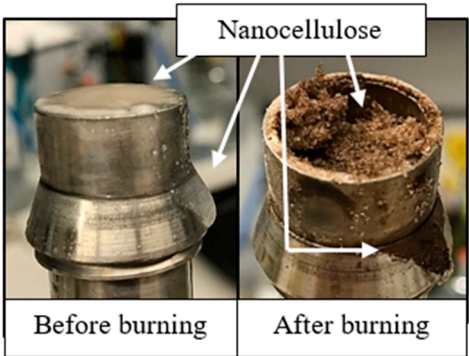
Figure 15. Inlet of sandpack flooded by 0.5 wt % CNC (USDA) in 1.0 wt % NaCl. Areas containing nanocellulose produced black ash after baking.
