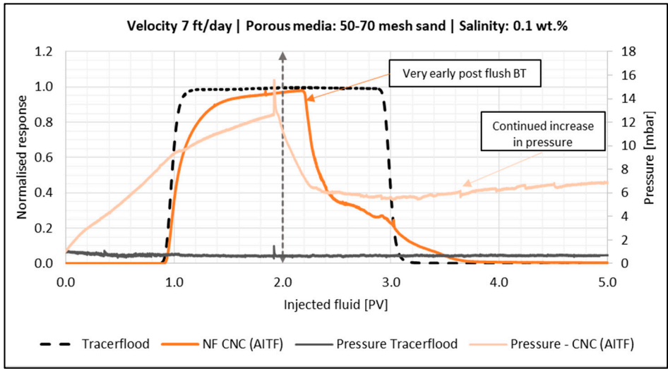
Figure 10. Breakthrough curve for the sandpack flood with 0.5 wt % CNC (AITF) (dark orange line) using a low velocity (7 ft/day). Dashed vertical line illustrates the switch to post flush fluid. The tracer BT-curve is the black dotted line. The corresponding pressure curves are also shown.
