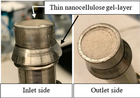
Figure 13. (Left) Inlet side of sandpack flooded with 0.5 wt % CNC (USDA) in 1.0 wt % NaCl. Thin film of nanocellulose gel sits on the top of the sand. The gel droplet (black arrow) came there as a result of opening the pack. (Right) Outlet side of the same pack after the flood shows no trace of nanocellulose, confirming that filtration prevented transport through the pack.
