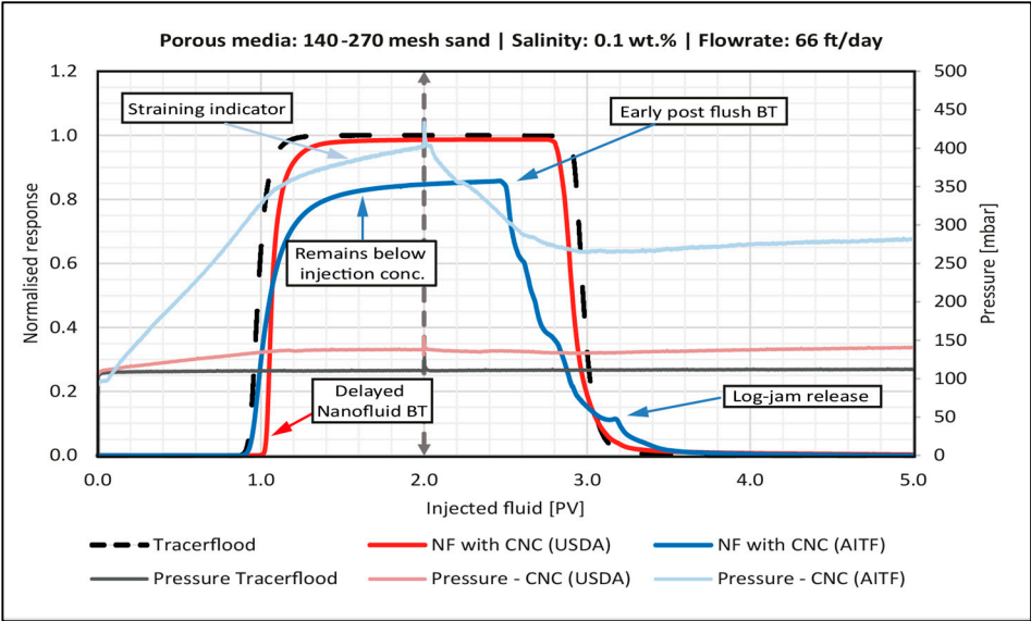
Figure 9. Breakthrough curve for the sandpackflood with 0.5 wt % CNC (USDA) (red line) and 0.5 wt % CNC (AITF) blue line. Dashed vertical line illustrates the switch to post flush fluid. The tracer BT-curve is the black dotted line.
