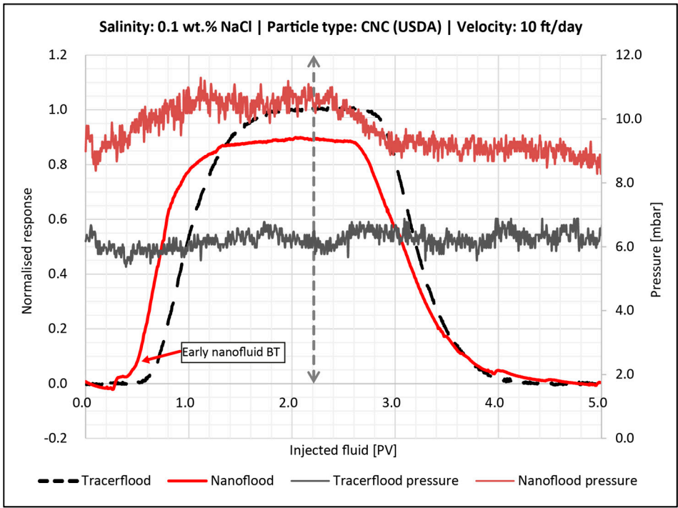
Figure 16. Breakthrough curve for the core flood with 0.5 wt % CNC (USDA) in 0.1 wt % NaCl (red line). 2.2 PV were injected followed by 0.1 wt % brine. The dashed vertical line illustrates when post flush was started. The tracer BT-curve is the black dotted line. The corresponding pressure curves are also shown.
