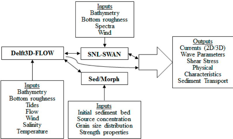
Figure 1. Flow chart illustrating the coupled Delft3D-FLOW-SNL-SWAN wave, circulation, and sediment transport models.
