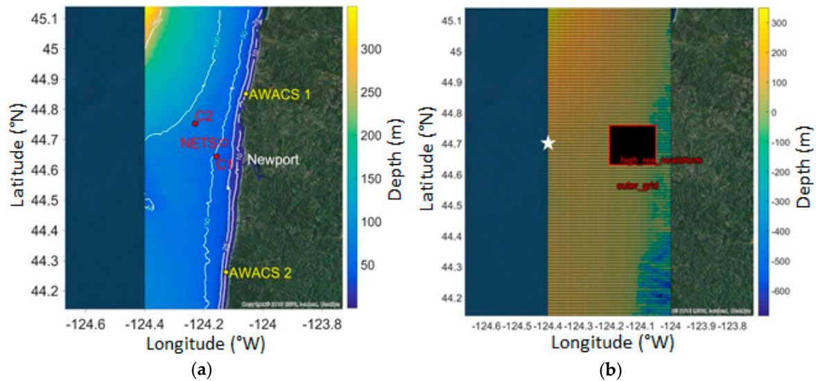
Figure 2. (a) Coupled Delft3D-FLOW-SNL-SWAN model domain and locations of available measurements; (b) Nested model grids. The star indicates the location of the NOAA NDBC buoy station 46089.
