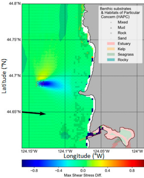
Figure 8. Same as Figure 7 but showing model results for winter conditions, where input wave parameters are H_s = 2.16 m, T_p = 10 seconds, D_p = 277^\circ .
