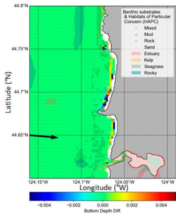
Figure 10. Same as Figure 8 but showing normalized changes in bed elevation, where Bottom Depth Diff. = \frac{h_w - h_b}{\max(|h_w - h_b|)} .
