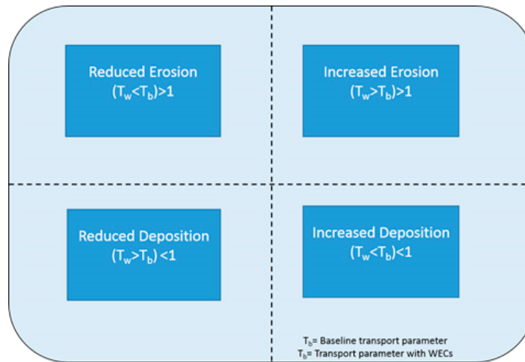
Figure 6. Sediment mobilization regimes associated with the relationship between the transport parameter for baseline (no WECs) and WEC scenarios, T_b and T_w , respectively (Eq. 2 and 3).
