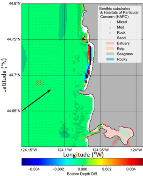
Figure 9. Same as Figure 7 but showing normalized changes in bed elevation, where Bottom Depth \text{Diff.} = \frac{h_w - h_b}{\max(|h_w - h_b|)} .
