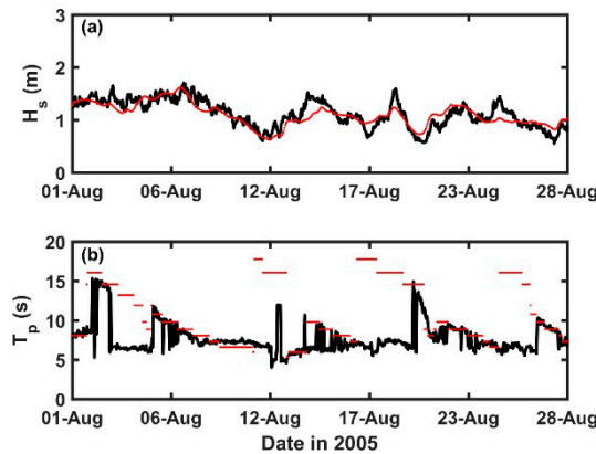
Figure 4. SNL-SWAN model validation results comparing (a) significant wave height and (b) peak wave period. Measured data from the OSU AWAC are shown in black and SNL-SWAN model data are shown in red.
