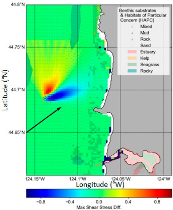
Figure 7. SEAT coupled numerical model results showing normalized changes in bottom shear stress for input waves typical of summer conditions, where Max. Shear Stress Diff. = \frac{\tau_w - \tau_b}{\max(|\tau_w - \tau_b|)} . Input wave model parameters were H_s = 1.37 m, T_p = 15 s, and D_p = 224^\circ . The black arrow indicates peak wave direction and the location of the WEC array is show by red crosses. Also shown are various benthic substrates and habitats of particular concern (HAPC; [17]).
