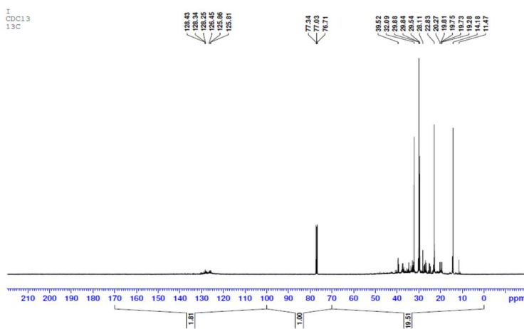
Figure 2. ^{13}\text{C} NMR spectra of the diesel fraction boiling at 200-350 °C.
