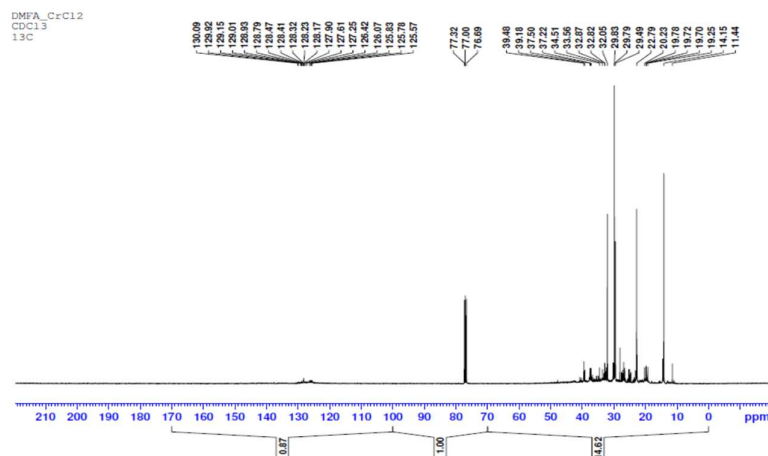
Figure 3. ^{13}\text{C} NMR spectra of the desulfurized diesel fraction 200-350 °C.
