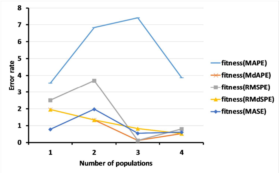
Figure 7. Material cost error rate.
