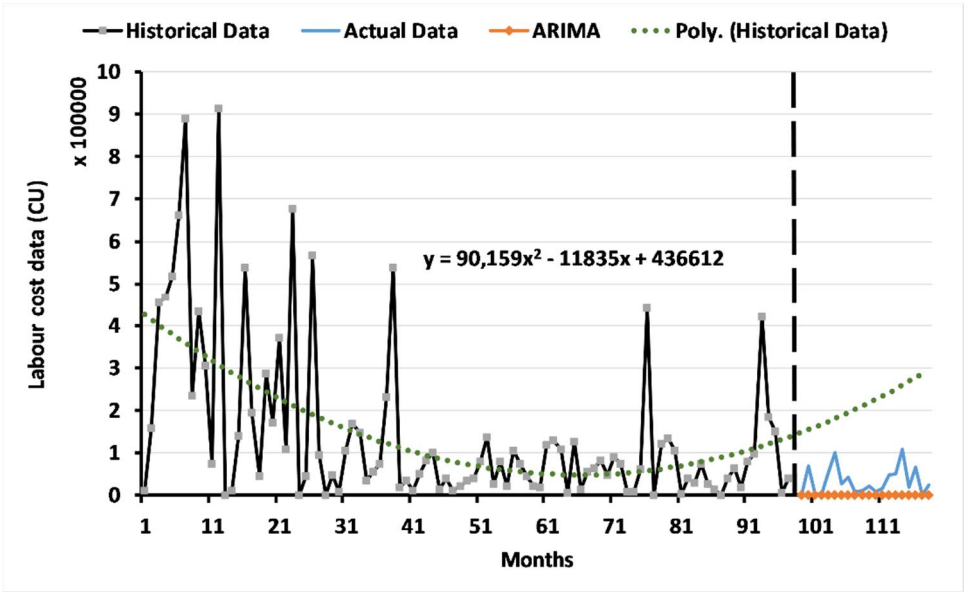
Figure 2. Labour cost data forecasting based on the ARIMA model.
