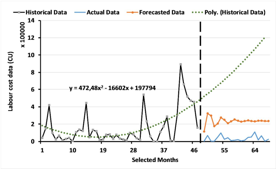
Figure 8. Labour cost data forecasting based on the dynamic regression model.
