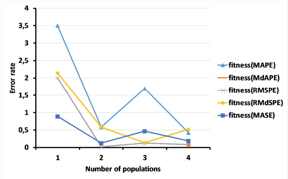
Figure 6. Labour cost error rate.
