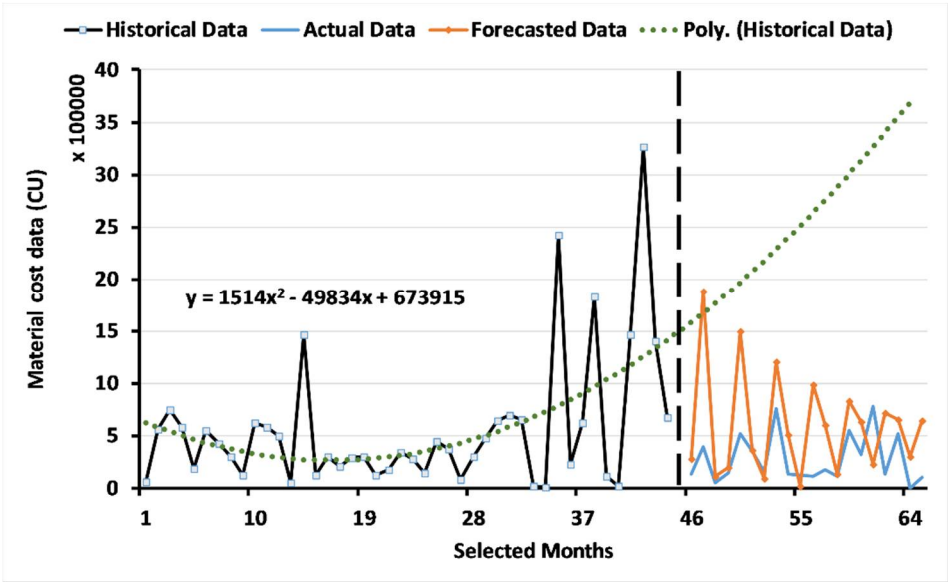
Figure 9. Material cost data forecasting based on the dynamic regression model.
