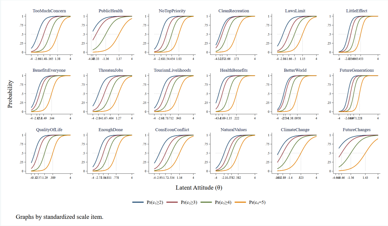
Figure 8. Item (boundary) characteristic curves. Each curve displays the cumulative probability of each item ordinal state. Dotted reference lines show scale values above which the cumulative probability exceeds 50%.
