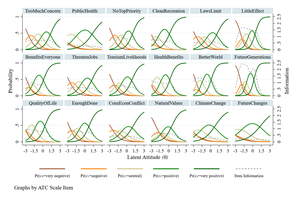
Figure 9. Item characteristic curves for the latent scale Attitudes toward coral reef conservation. Colored lines denote varying response curves to signed item characteristics. Dotted lines display information characteristics curves for each scale item.
