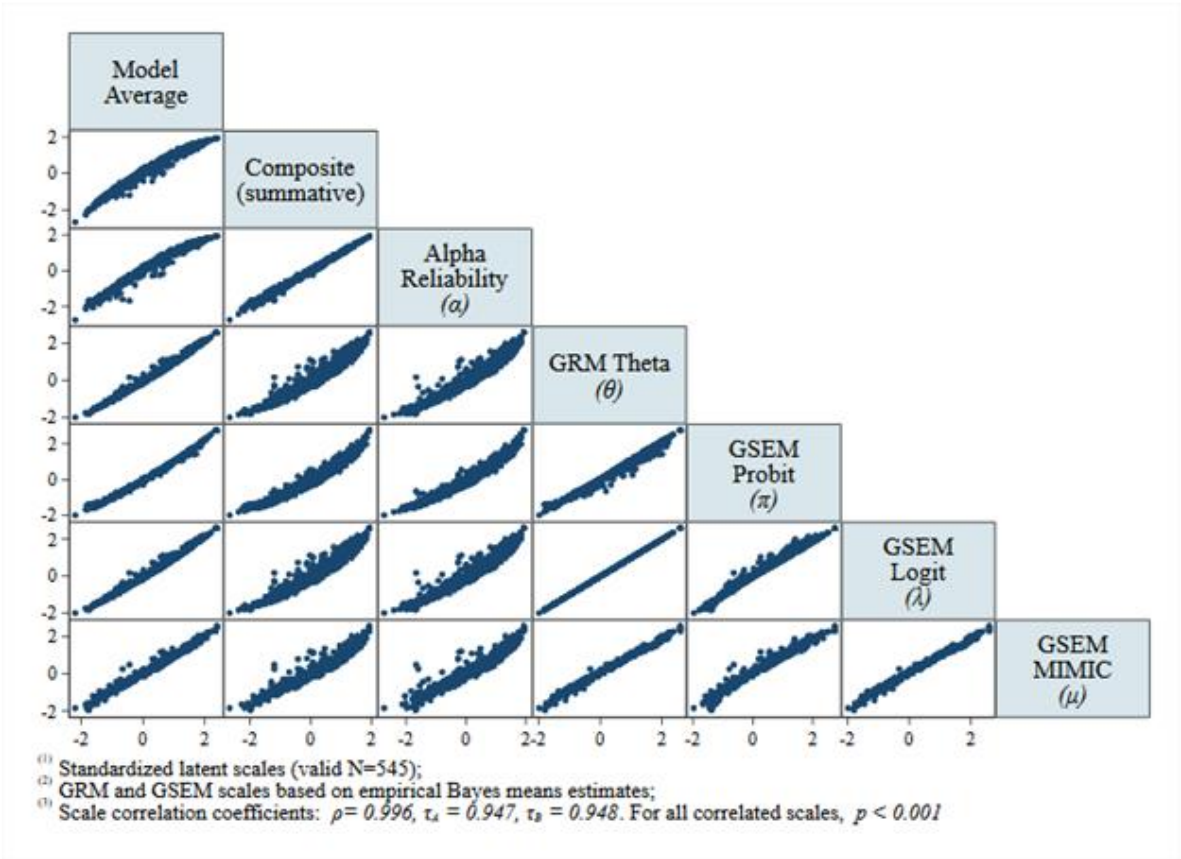
Figure 11. Congruency visualization among ATC latent trait scale estimations.
