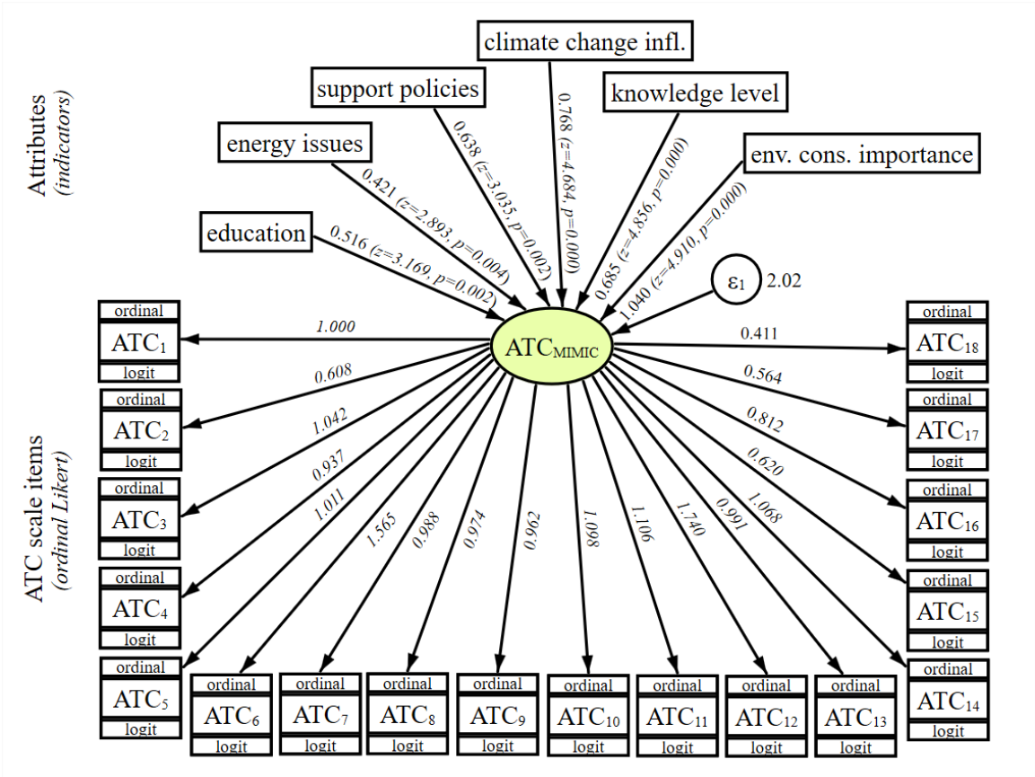
Figure 10. Graphical representation of the estimated GSEM MIMIC model parameters for the ATC latent attitudinal scale. The MIMIC model uses an ordinal logit fit for the 18 scale item parameters, adjusting for covariance contributions from a number of associated attributes (6 attributes). The fitted mean values of the estimation (along with z-scores and p-values for the attributes) are shown alongside the connecting arrows.
