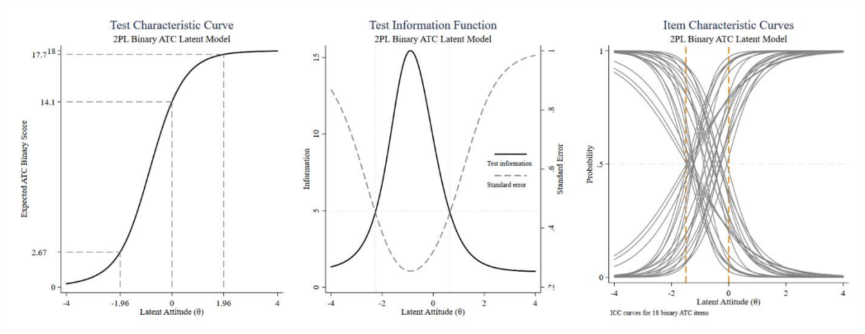
Figure 6. Test, information, and item characteristic curves of the 2PL IRT latent ATC model estimation. The left subgraph plots the cumulative test characteristic curve of the model. The dotted lines indicate corresponding 95% probability boundaries. The center subgraph plots the overall test information function (solid line) and the standard error of the information estimate (dotted line). The right subgraph plots all 18x2 item characteristic curves (binary). The dotted reference lines indicate boundaries of latitude of non-commitment area.
