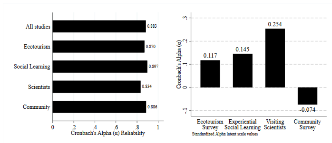
Figure 1. Standardized Cronbach's alpha reliability estimated for the optimal implementation of the ATC latent scale. The bars on the left subgraph show standardized alpha coefficients by study strata, while the bars on the right subgraph show differences in mean scale coefficients of each study strata from the overall latent scale (for all studies).
