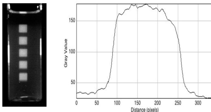
Figure 7. Left: A 20 mm square cell containing a 60 mm length of an RFG gel irradiated 5 times with a 5 mm square X-ray beam (dose 10 Gy) with the beams vertically displaced by 10 mm between irradiations. Right: A pixel profile scan across the central beam at 0.030 mm per pixel.
