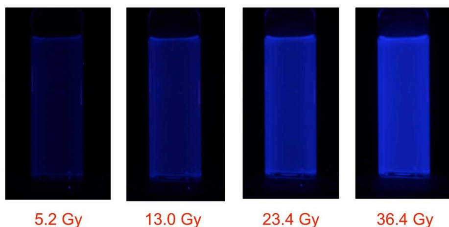
Figure 2. Upper: The full RGB color fluorescence in UV light of a 10x10 mm 2 cuvette containing a 1.4 mM solution of maleimido-pyrene in tertiary-butyl acrylate, as a function of accumulated dose in a GC200 \gamma -ray source (dose rate \sim 2 Gy/min). Lower: The same cuvette with the fluorescence show as blue-pixel gray-scale values.
