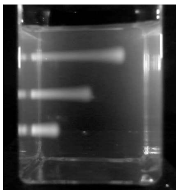
Figure 13. 80 MeV proton beam tracks imaged in a 40x40x40 mm 3 RFG gel; attenuated, from top to bottom, by polystyrene sheets 22, 32 and 42 mm thick. Portal dose 15 Gy.
