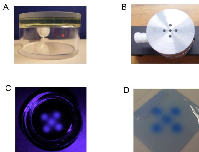
Figure 3. The first test measurement of fixed fluorescence imaging using the RFG gel production procedure described in the text. A. A cylindrical spectrosil cell containing a (slightly yellow) 5mm layer of a quasi-rigid gel containing ~1 mM MPy in TBA/15%PTBA. B. The 5mm thick aluminium mask for collimating the 3 MeV electron beam. C. The fluorescent image of the gel in 365 nm light after irradiation with a dose of 20 Gy. D. Comparison with a radio-chromic film irradiated under the mask to 10 Gy.
