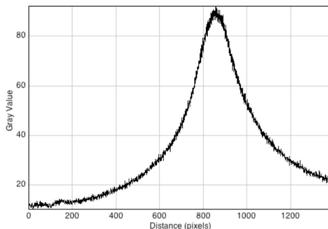
Figure 16. A pixel profile scan taken along the axis of the catheter, i.e. the vertical axis in Figure 15. The pixel resolution is 0.035 mm/pixel with a total scan length of approximately 50 mm.
