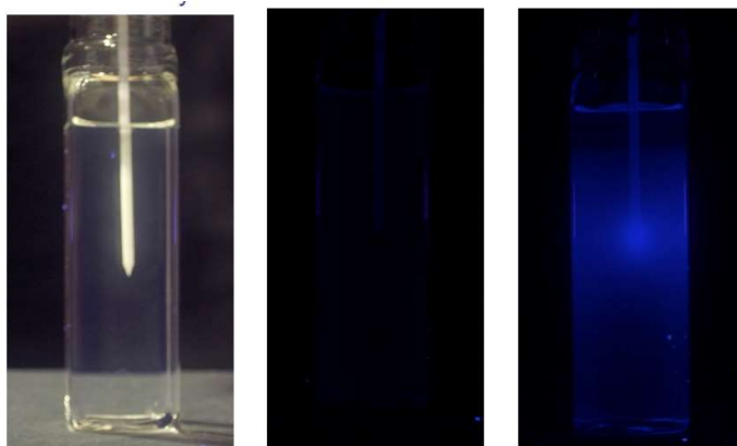
Figure 14. The set-up used to monitor, in situ , the fluorescence of an RFG gel on insertion of a seed of ^{192}\text{Ir} . The main constituents are a 20 \times 20 \text{ mm}^2 glass cell containing the gel into which a 1.9 mm diameter catheter (shown in Figure 15) is inserted via a septum cap ; two mercury-arc UV (365 nm) lamps, a Ricoh GX200 digital camera with a lead shield against gamma irradiation and wooden shields against direct UV.
