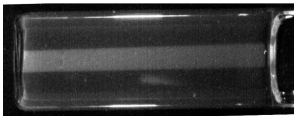
Figure 8. The image of a 5x5 mm 2 200 kVp X-ray beam propagating in a 60 mm length of RFG gel contained in a 20x20 mm 2 cell. Optical artifacts occur at the glass/air sides of the cell and at the gel meniscus.
