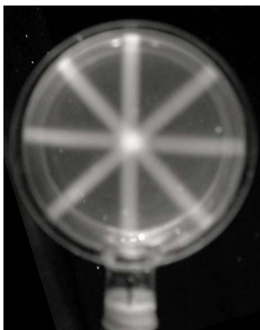
Figure 10. The fluorescence of a 6 mm thick RFG gel in a 50 mm diameter cylindrical quartz cell after irradiation with a 2.5 mm collimated, 250 kVp X-ray beam at 0, 45, 90 and 135 degrees to the vertical.
