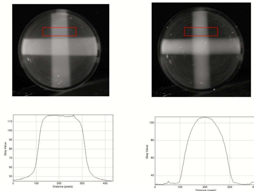
Figure 11. A 20 mm thick RFG gel irradiated with orthogonally-crossed X-ray beams. Upper left; a 10x10 mm square beam, Upper right; a 10 mm diameter round beam. Lower; pixel profiles across the beams as shown by the red rectangles. Pixel resolution 0.049 mm/pixel.
