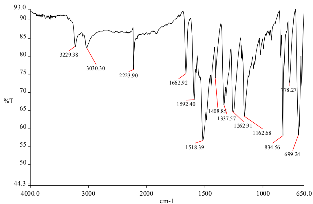
Figure S1. The FT-IR spectrum of N-benzoyl-N'-(2-cyanophenyl)thiourea
