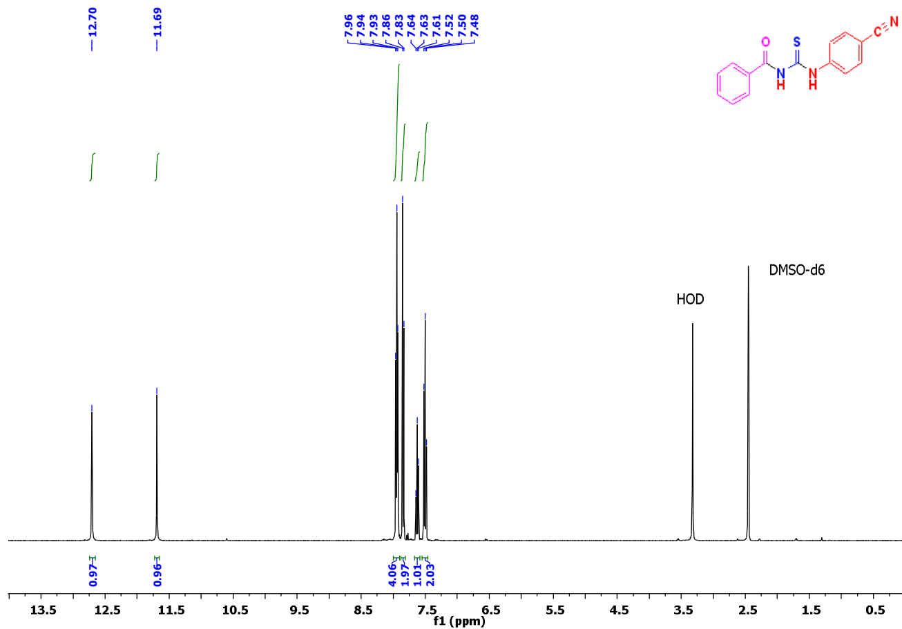
Figure S3. The 1 H-NMR spectrum of the N-benzoyl-N'-(2-cyanophenyl)thiourea
