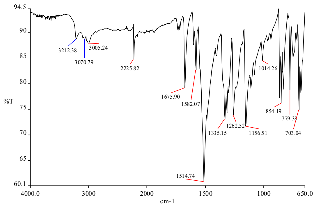
Figure S2. The FT-IR spectrum of N-(4-nitrobenzoyl)-N'-(2-cyanophenyl)thiourea.
