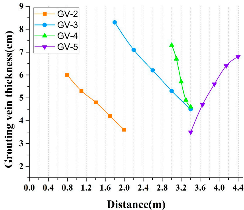
Fig 16. Measured value of the grouting veins
