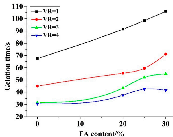
Fig 8. Test result of gelation time of the slurry
