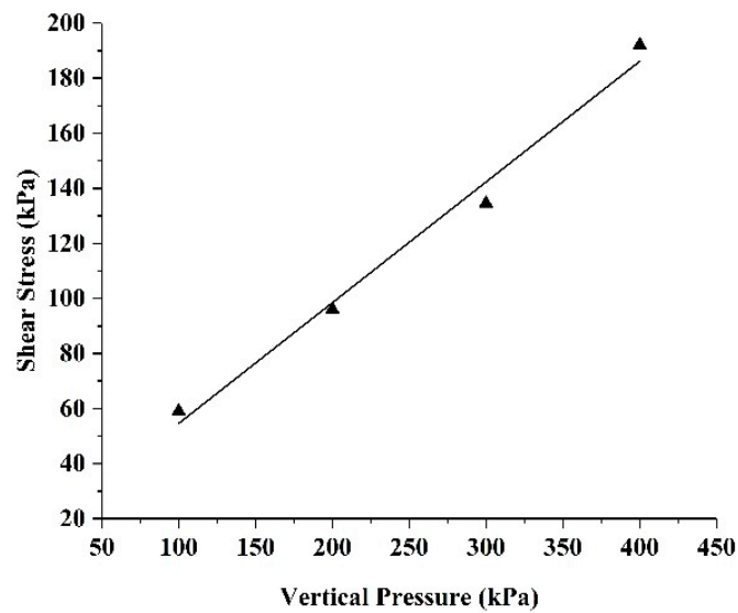
Fig 2. Result of direct shear test
