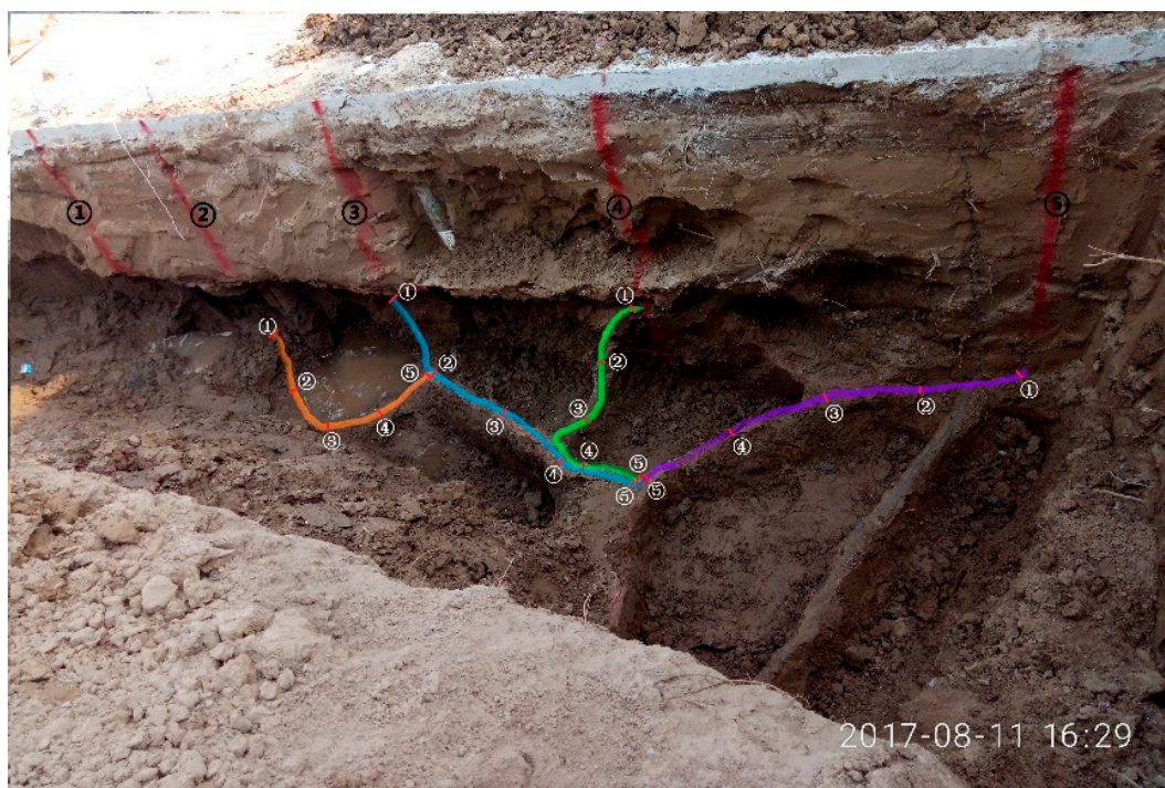
Fig 15. Pit prospecting result
