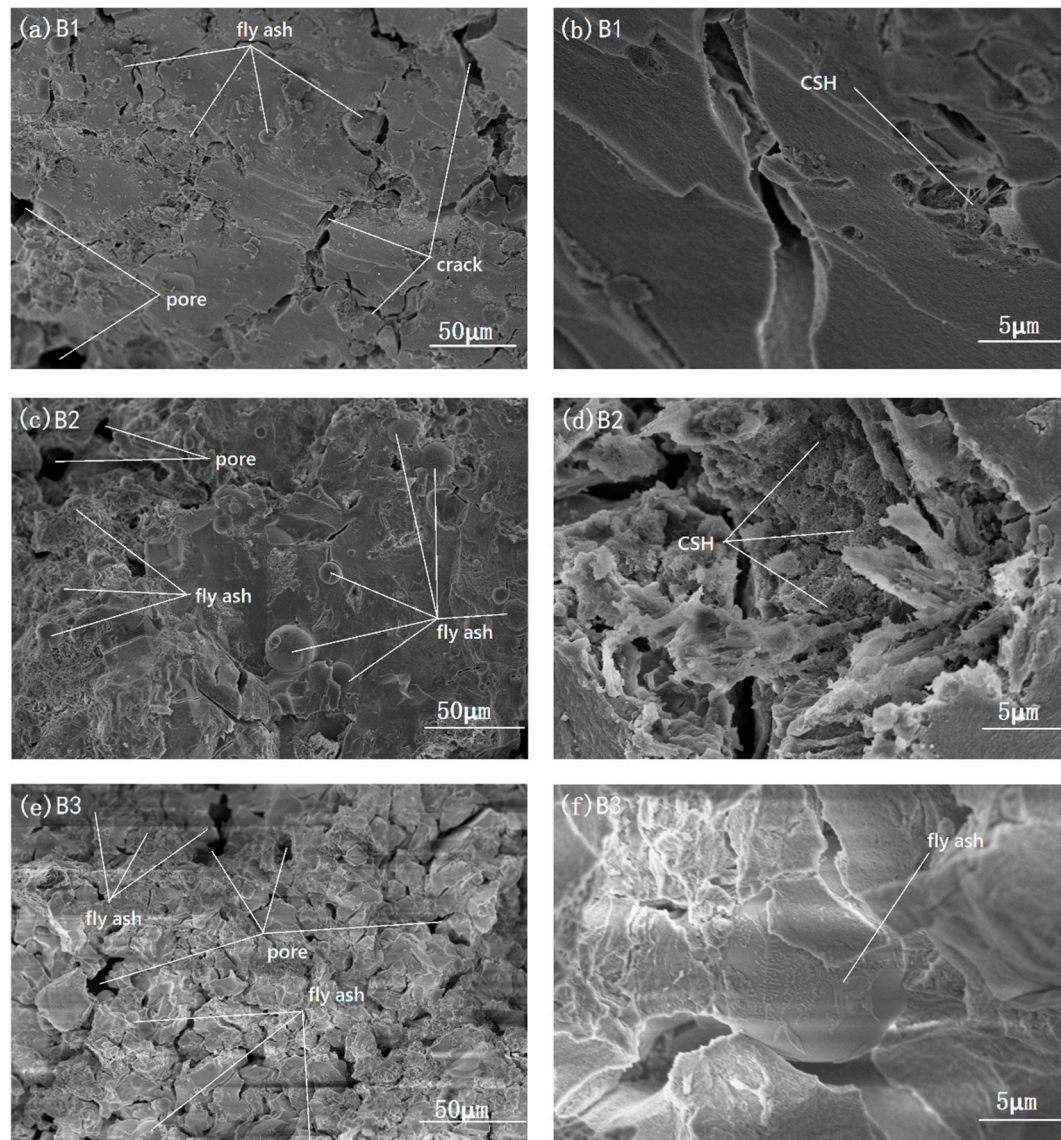
Fig 10. Photographs of SEM of the specimens under different fly ash content
