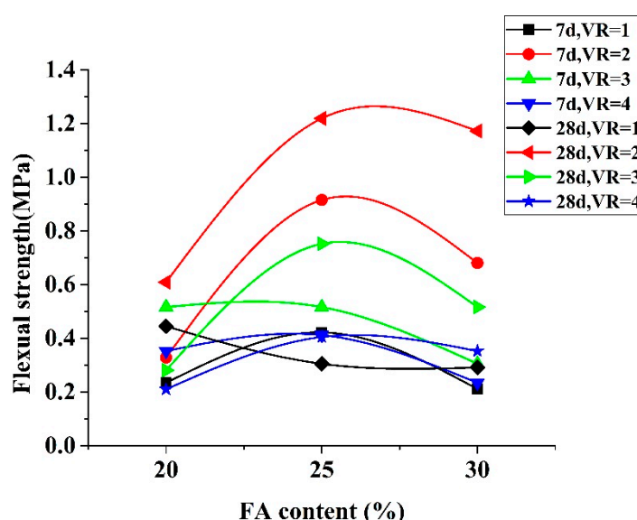
Fig 9. Test result of flexural strength of the specimen
