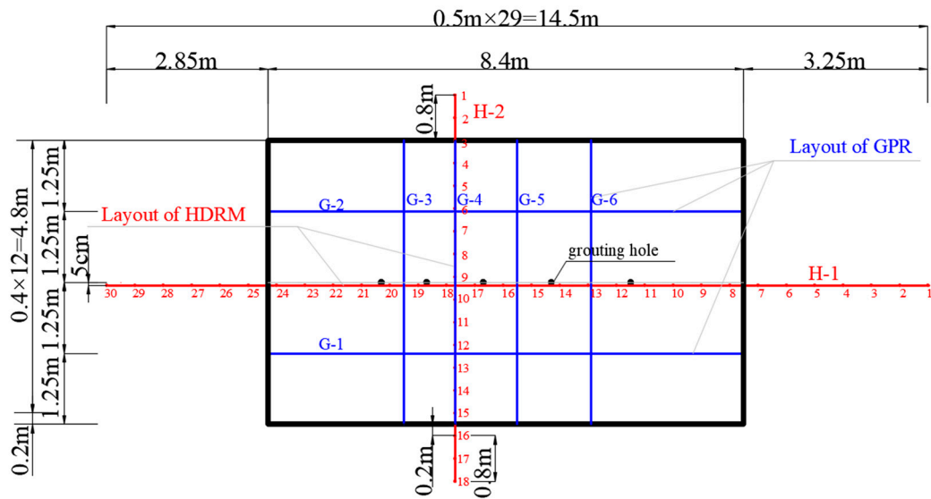
Fig 7. The layout of GPR and HDRM
