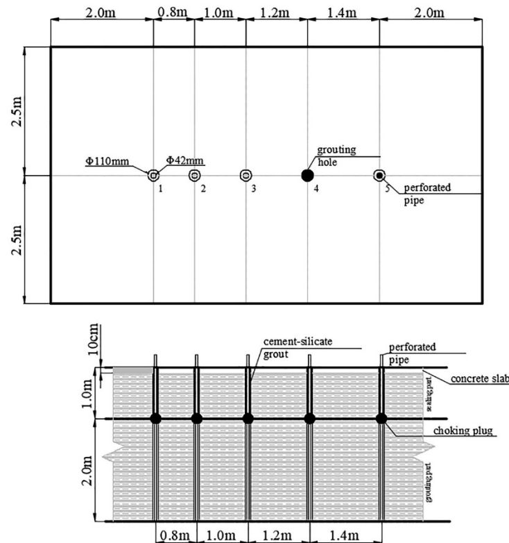
Fig 3. Layout of field test
