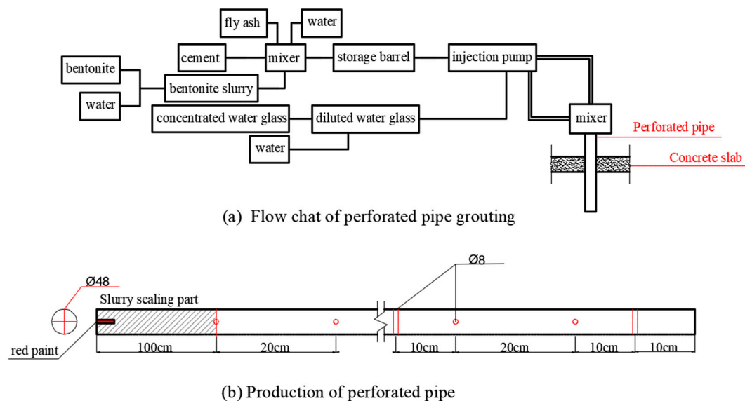
Fig 4. Flow chat of perforated pipe grouting and production of perforated pipe
