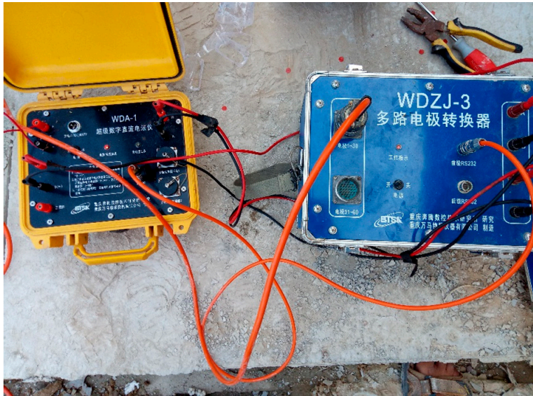
Fig 6. High Density Resistivity Method
