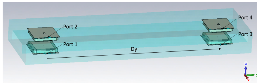
Figure 6. Four patch antennas placed on the entrance housing. Patch antennas are fed by a coaxial probe. The antenna size is 50 \text{ mm} \times 50 \text{ mm} \times 6.5 \text{ mm} .
