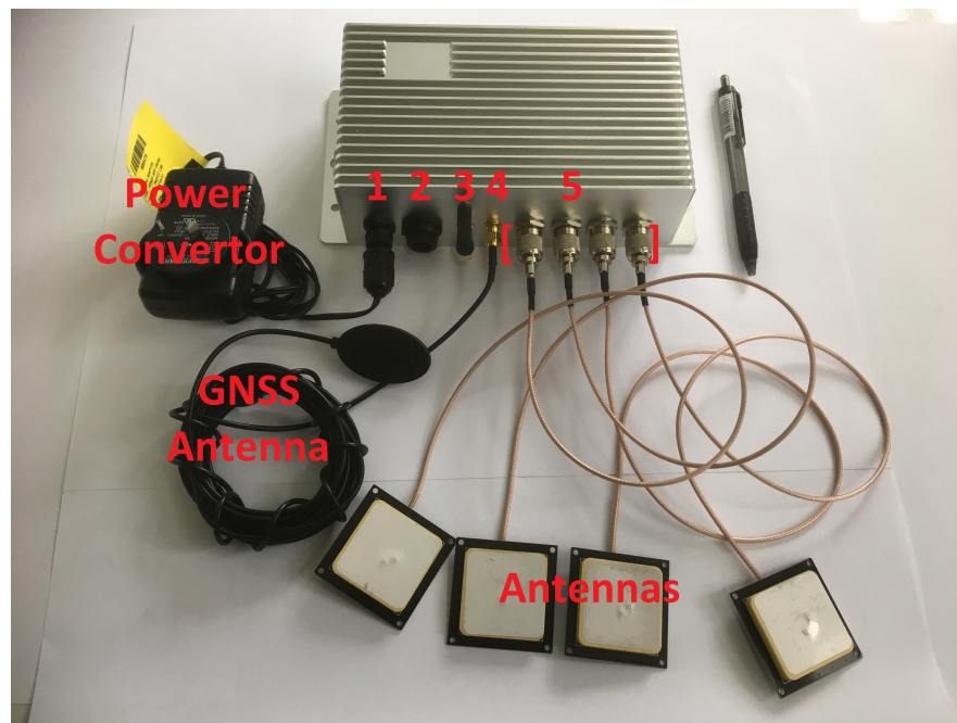
Figure 3. Aluminum housing (18.5 cm × 10.5 cm × 5.5 cm) and peripherals. 1) 4-pin power inlet; 2) micro-USB port; 3) Wi-Fi antenna, and 5) RFID antennas and ports.
