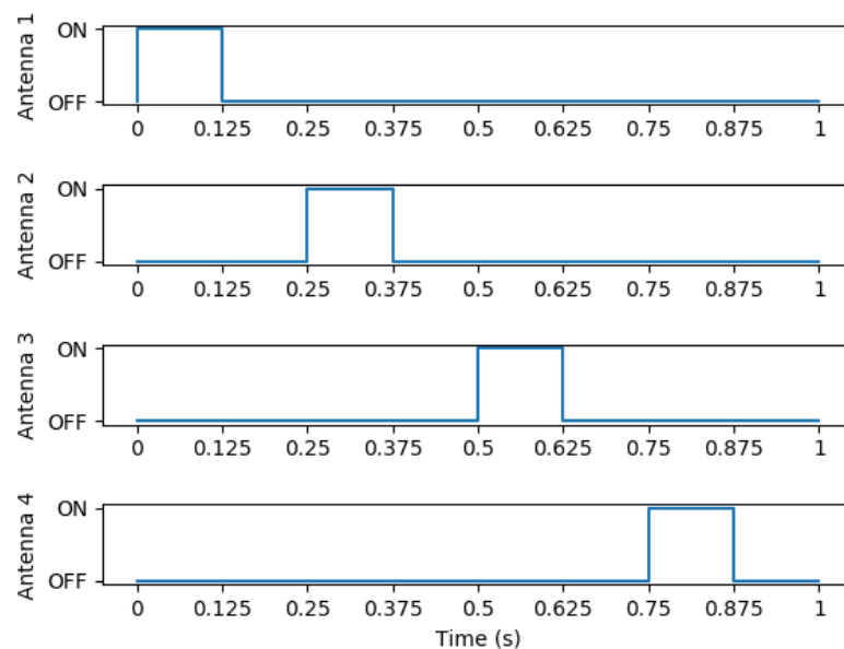
Figure 8. The structure of a duty cycle of the RFID reader operation. It is only possible to power one antenna at a time and all antennas must be off for a given time as well. The time span during which each pair of antennas (Figure 5) operate can be tailored to how fast the bee species under study moves.
