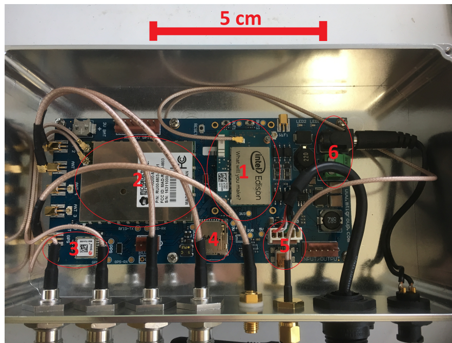
Figure 2. Printed Circuit Board showing the main components: 1) IoT module; 2) HP-SiP module; 3) GNSS receiver; 4) micro-SD card; 5) micro-USB I/O; and 6) power regulator.
