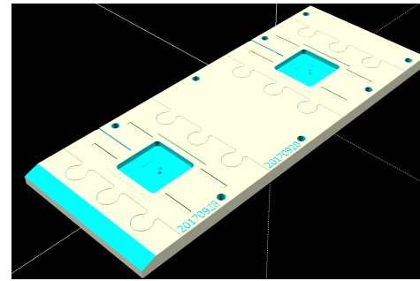
(b) Internal view of entrance housing. This is mirrored by the opposite layer of the housing to provide matching pairs of antennas. The centers of the highlighted squares (where the antennas are mounted) are 17 cm apart.
