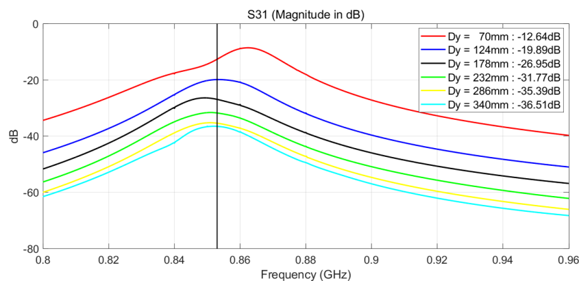
Figure 7. Simulated S31 versus distance Dy for the configuration of the antennas shown in Figure 6. Distance Dy is measured between the centres of patch antennas.
