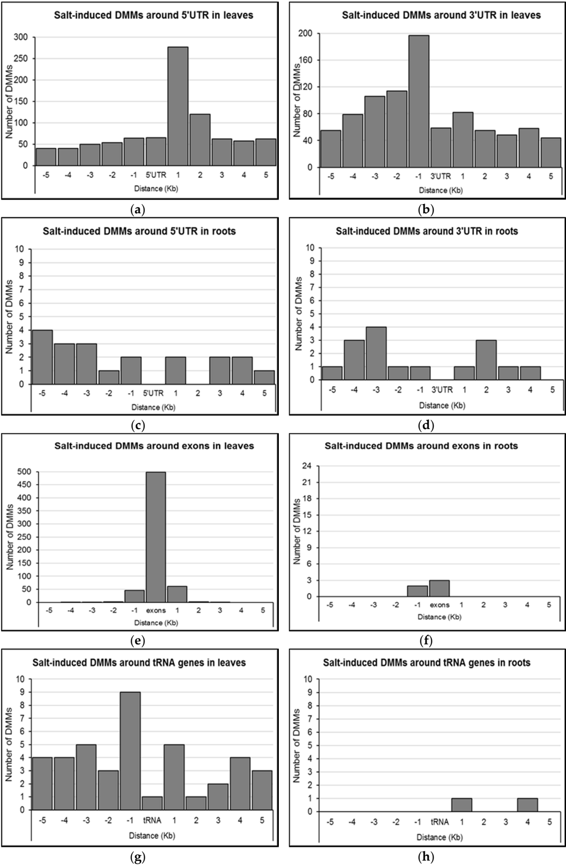
Figure 6. Distribution of salt-induced differentially methylated markers (DMMs) around UTRs, exons and tRNA genes. (a,b) 5'UTRs and 3'UTRs in leaves; (c,d) 5'UTRs and 3'UTRs in roots; (e) exons in leaves; (f) exons in roots; (g) tRNA genes in leaves; (h) tRNA genes in roots. The distance of each
