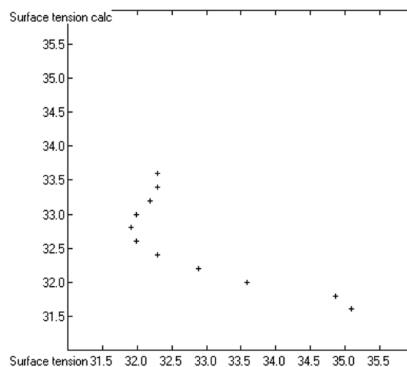
Fig. 4h: 1-( \text{CH}_3(\text{CH}_2)_n )-3-methylimidazolium
