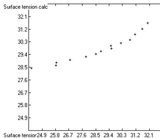
Fig. 4d: 1-Bromo-n-alkanes
