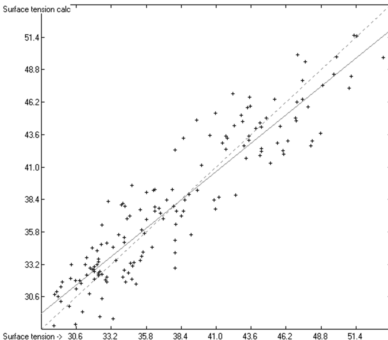
Figure 3. Correlation Diagram of the Surface-Tension Data of the Ionic Liquids. (N = 154; R^2 = 0.8579 )
