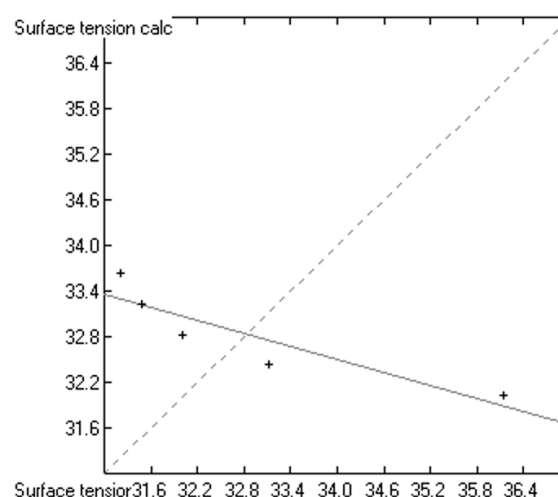
Fig. 4f: 1,4-Bis( \text{CH}_3(\text{CH}_2)_n\text{COO} )-2-butyne,
