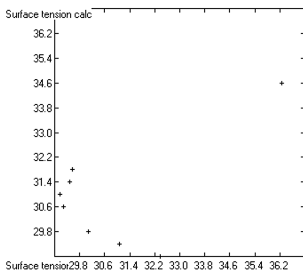
Fig. 4g: 1,3-Bis( \text{CH}_3(\text{CH}_2)_n )imidazolium
