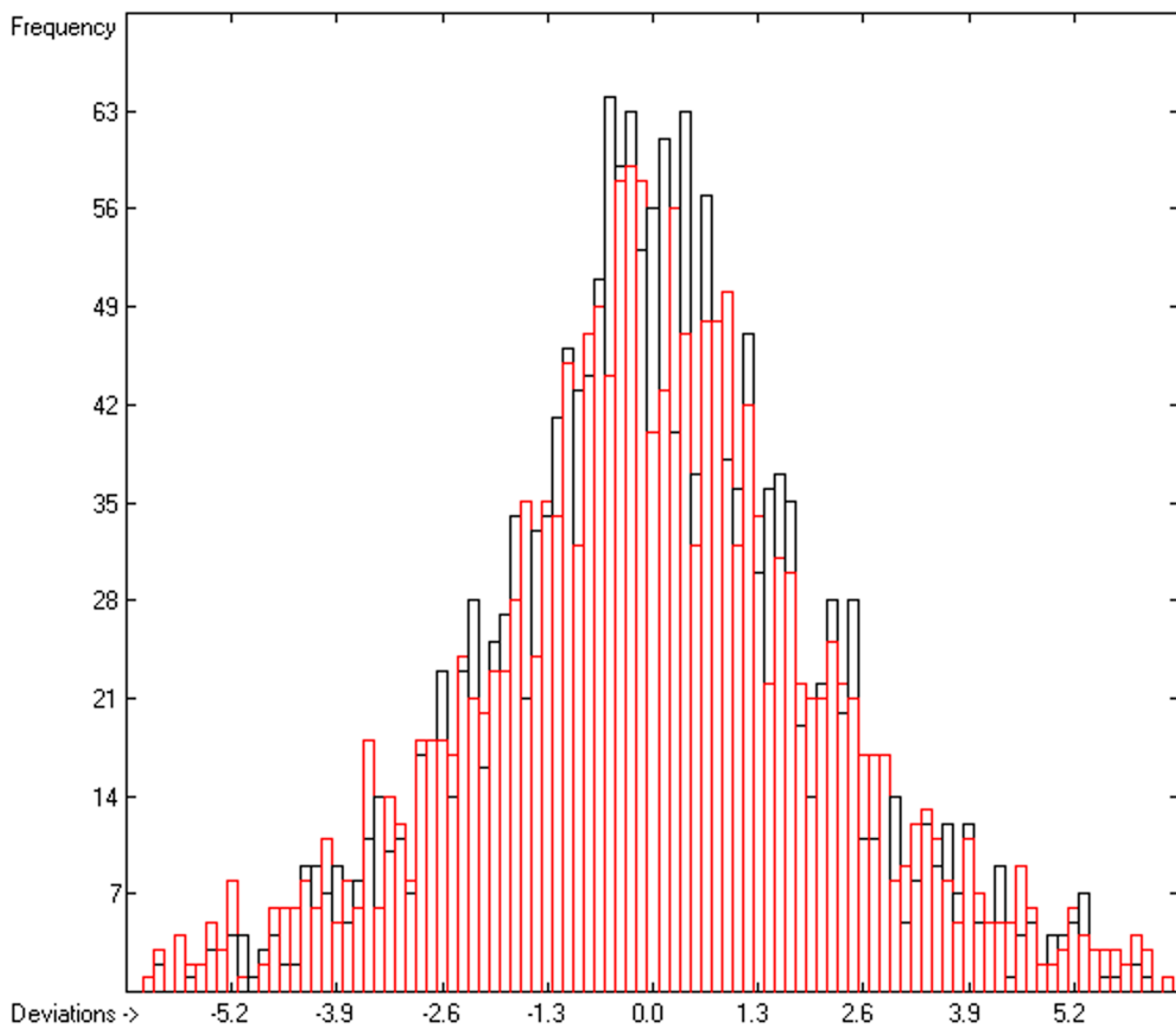
Figure 2. Histogram of the Surface-Tension Data. Cross-validation data are superpositioned as red bars. ( S = 2.16 ; experimental values range: 9.89 – 53.5)
