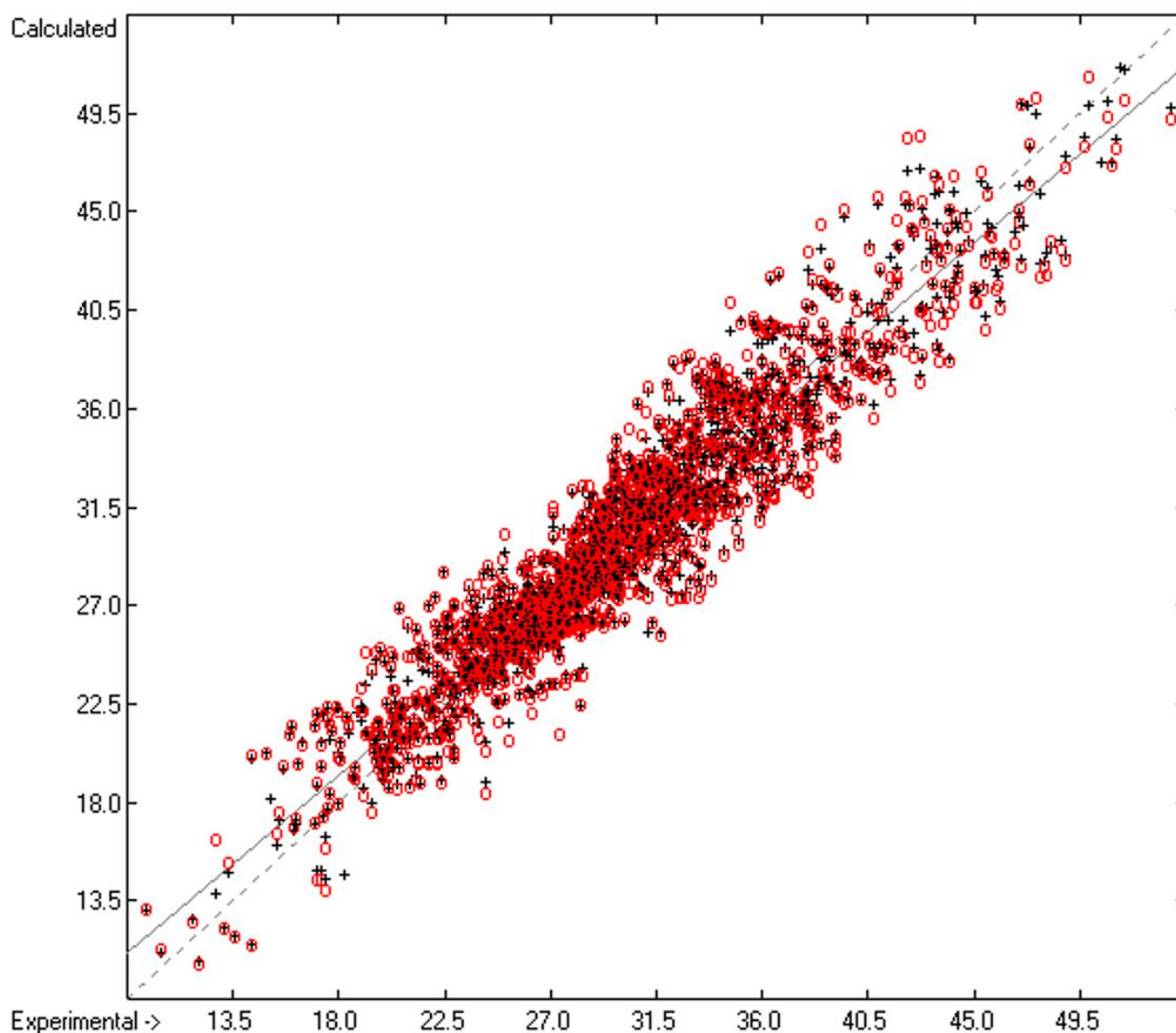
Figure 1. Correlation Diagram of the Surface-Tension Data. Cross-validation data are added as red circles. ( N = 1835 ; R^2 = 0.9024 ; Q^2 = 0.8821 ; regression line: intercept = 2.9750; slope = 0.9017)
