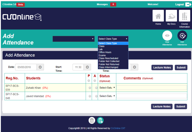
Fig. 6: Attendance System
