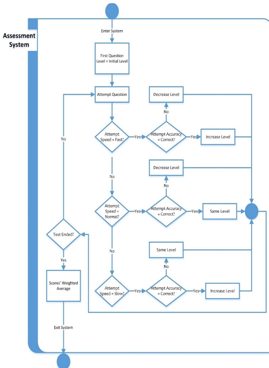
Fig. 17: Working Details of the Smart Assessment System
