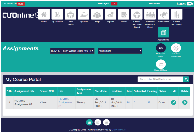
Fig. 9: Assignments Tab
