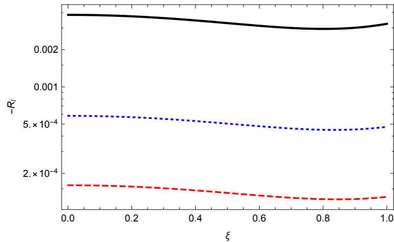
Figure 1. The ratio of the remainder contributions to the energy relative to the lowest order approximant, R_l/E^{(2)} for isorefractive dielectric-diamagnetic balls. Plotted are the negative of this ratio for l = 1 (solid, black), l = 2 (dotted, blue), and l = 3 (dashed, red).
