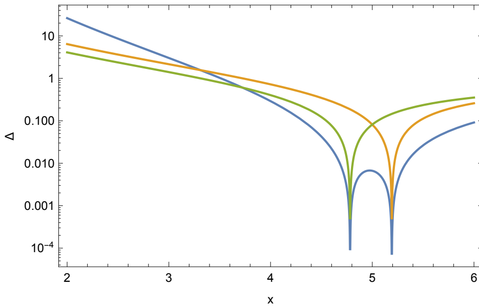
Figure 4. Zeroes of \Delta^E (right) and \Delta^H (left), and of their product, shown by the plots of their magnitudes, for l = 1 and \lambda = 10 . As \lambda gets large, the zeroes approach \lambda/2 for all l .
