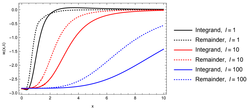
Figure 5. The integrand of the energy w_l(x, \lambda) given by (26) for \lambda = 1 and l = 1, 10, 100 , shown by the dotted lines. The solid lines show the unsubtracted \ln \Delta^E \Delta^H integrand. The removal of the leading UAE contributions greatly improves the large x behavior, but leaves large and growing contributions for moderate values of x .
