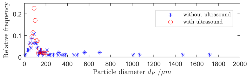
Figure 13. Comparison of the particle size distribution at dispersing flour with the system shown in figure 11c with and without using ultrasound
