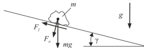
Figure 4. Resulting forces acting on a powder particle on an inclined plane
