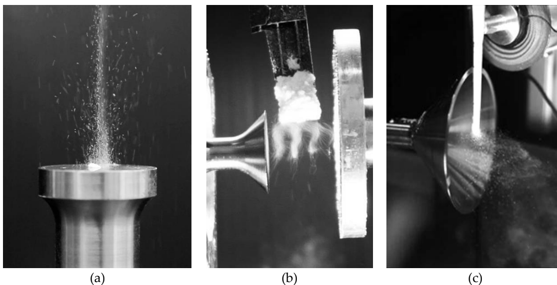
Figure 11. Principles for deagglomeration and dispersion of dry fine powders: (a) flour on vibrating sonotrode, f = 20 \text{ kHz} ; (b) flour in a standing ultrasonic wave, f = 46 \text{ kHz} ; (c) flour in a focused ultrasonic wave, f = 35 \text{ kHz}
