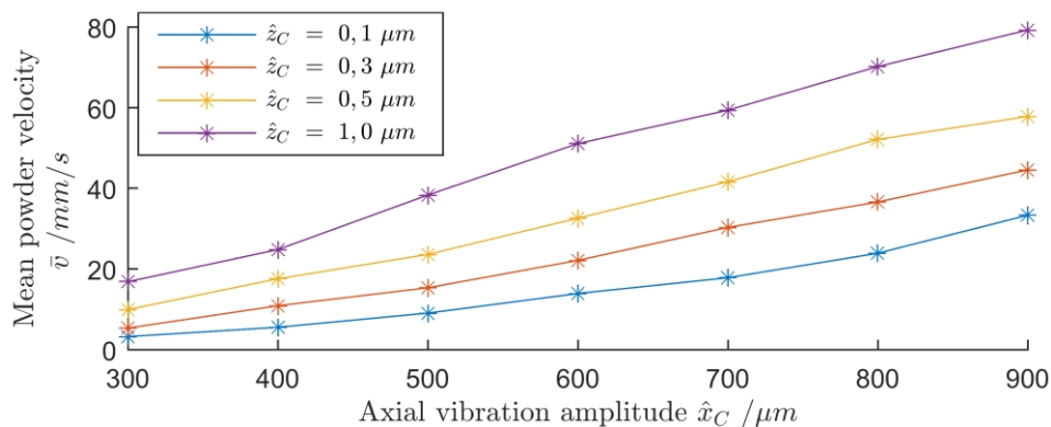
Figure 10. Mean powder velocity for variation of amplitudes of axial and radial excitation of the pipe; test powder: flour; frequencies f_a = 50 \text{ Hz} , f_r \approx 35 \text{ kHz}
