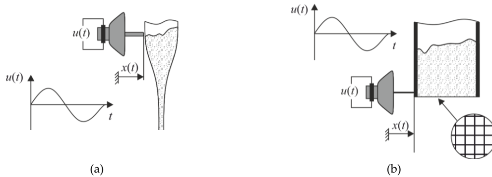
Figure 3. Dosing systems that use vibrations to enable powder flow; (a) glass pipette with knocking device, (b) cylindrical vessel with vibrating sieve at the outlet
