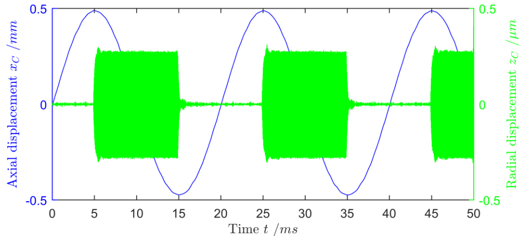
Figure 9. Axial and radial displacement of the pipe vibration in the powder transportation system; pipe material: aluminum alloy
