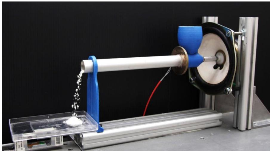
Figure 8. System using coordinated manipulation of friction forces for the transportation of dry flour.
