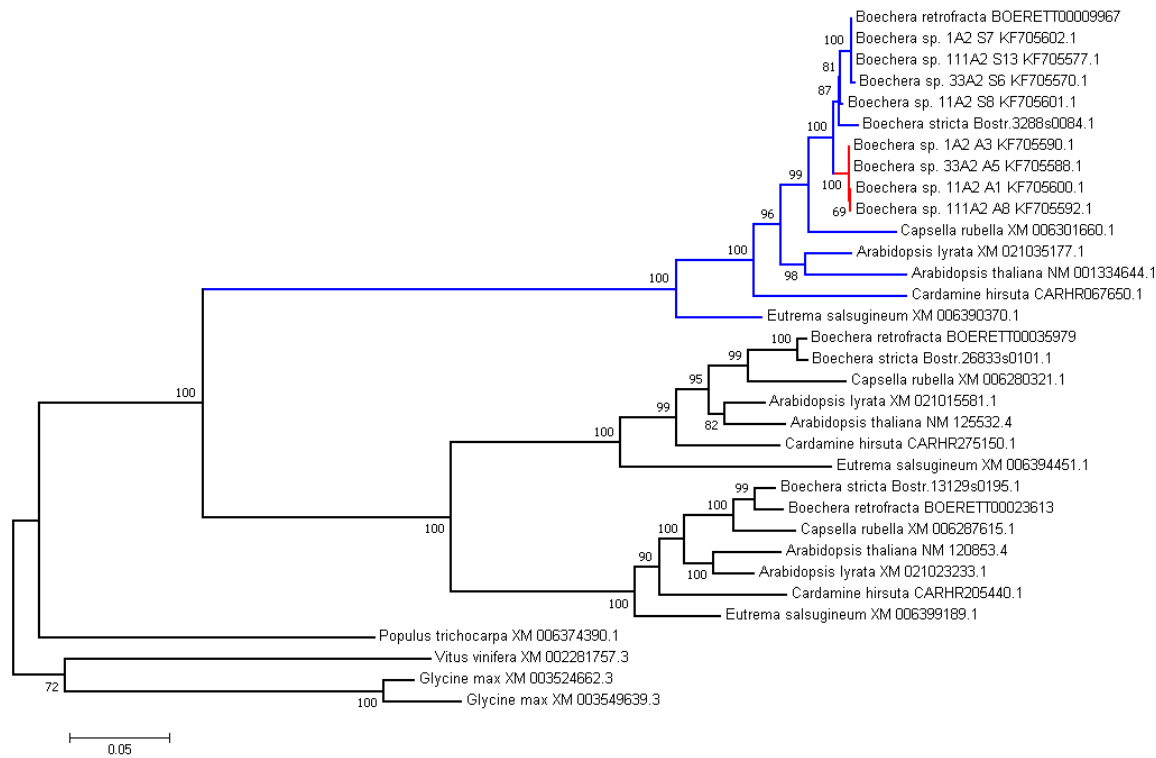
Figure 4. Phylogenetic tree of the isoforms of APOLLO locus (exonuclease NEN) in seven species of interest and alleles of APOLLO locus of apomictic Boechnera species from Corral et al (2013). Sequences of Populus trichocarpa , Vitus vinifera and Glycine max were used as outgroup. The clade related to the APOLLO locus is shown in blue, with apo-alleles shown in red.
