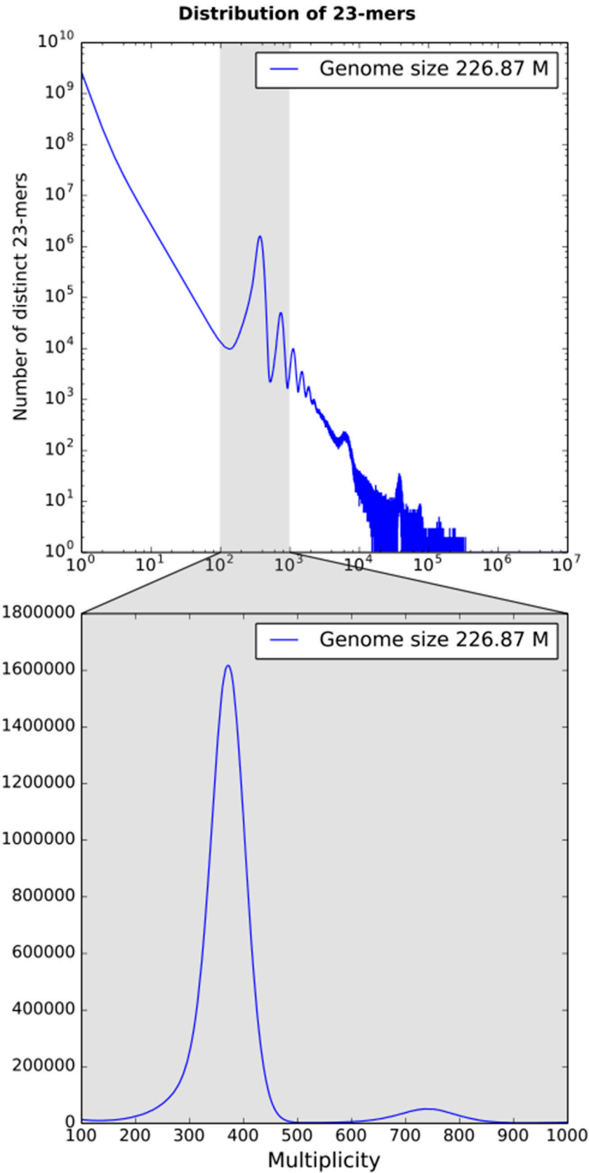
Figure 2. Distribution of 23-mers for PE LIB400 library. Only one major peak at 371x coverage is present, suggesting low heterozygosity (bottom plot), however there are detectable duplications and triplications at 737x and 1120x coverage (upper plot, Y axis is on a logarithmic scale).
