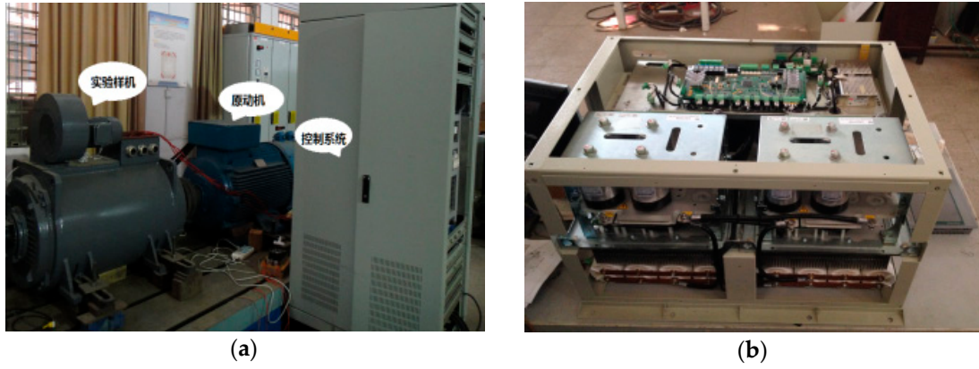
Figure . The photo of the experimental test rig system: (a) The experimental platform and power control cabinet; (b) The converter module and its controller.
