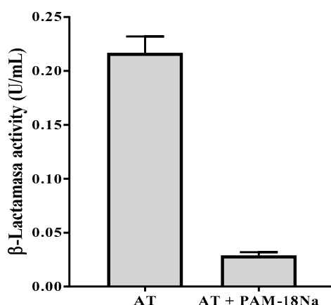
Figure 8. Effect of the polymer PAM-18Na on the activity of the P. fluorescens \beta -lactamase
