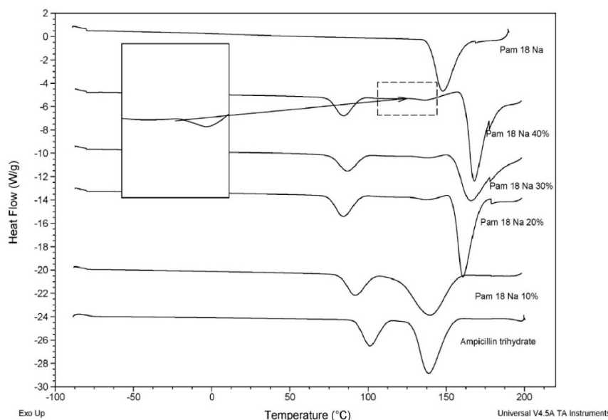
Figure 2. DSC Thermograms of ampicillin trihydrate and PAM-18Na polymer in solid blends at different proportions.
